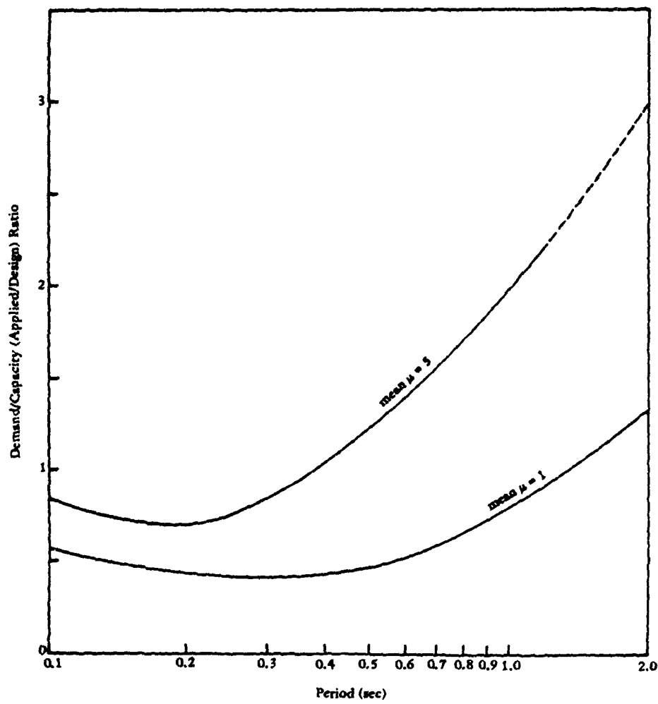
Figure C-7. Mean ductility.
