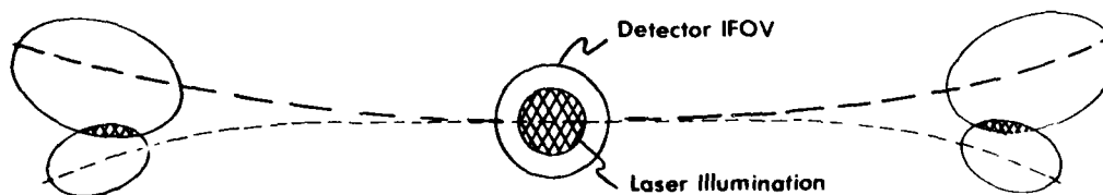
FIGURE 2-17. LOSS OF TRANSMITTER/RECEIVER REGISTRATION WITH INCREASING SCAN ANGLE
