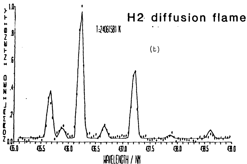
Figure 12. H 2 CARS spectra obtained in various environments using a 2300 groove/mm grating giving a resolution of about 5 cm -1 ; (a) pure H 2 at room temperature using BOXCARS geometry, (b) a H 2 diffusion flame using BOXCARS geometry.
