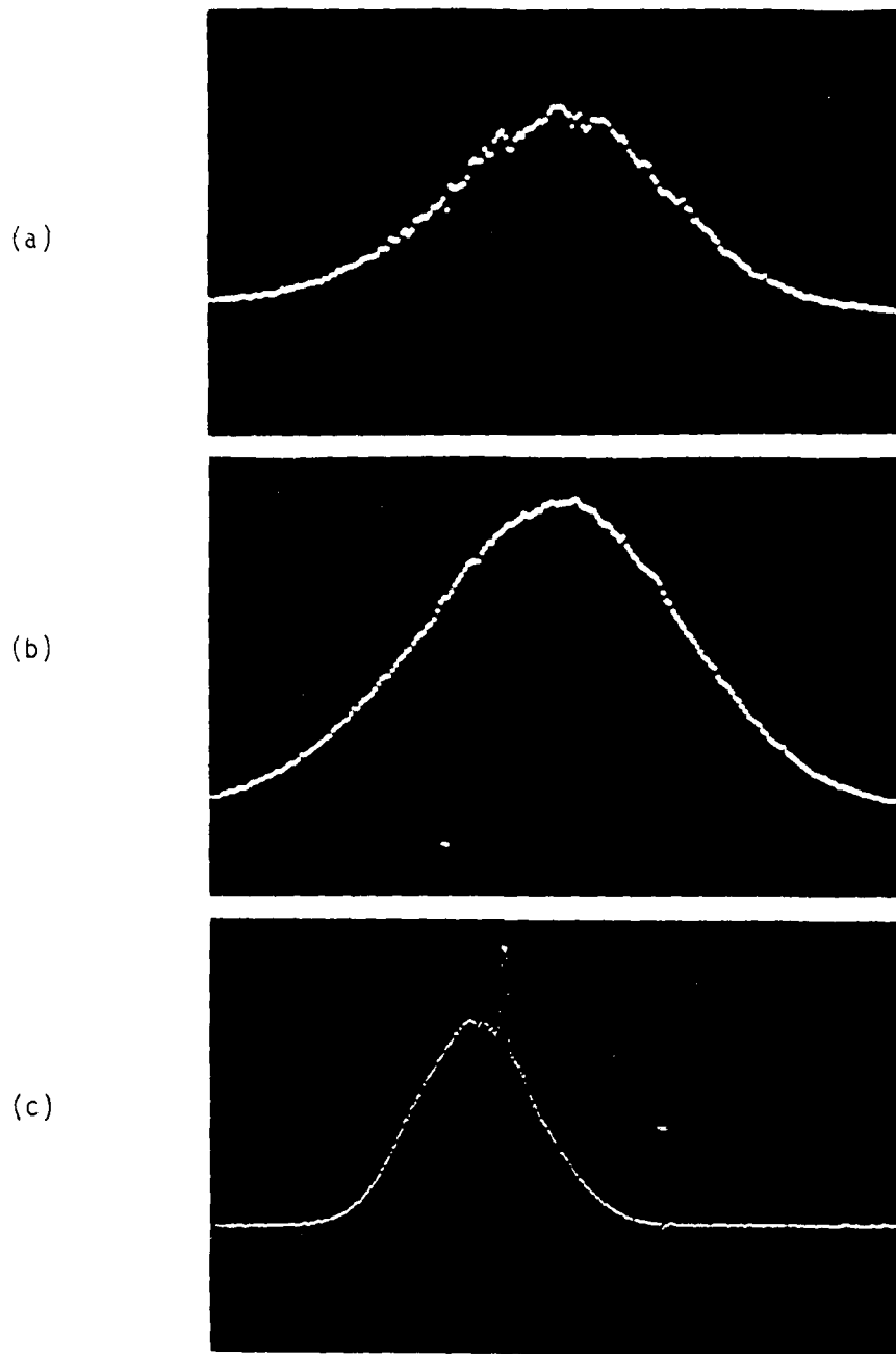
Figure 4. Frequency spectra of the dye laser. (a) Broadband dye laser output from a single laser shot. The peak is centered at 631 nm with a FWHM of about 110 \text{ cm}^{-1} . (b) Same conditions as in (a) except 16 laser shots were accumulated. (c) The dye laser was operated such that a broadband and narrowband output was produced simultaneously for the purpose of checking the center frequency. Here the narrowband output is 633 nm as indicated by the calibrated wavelength dial of the dye laser.
