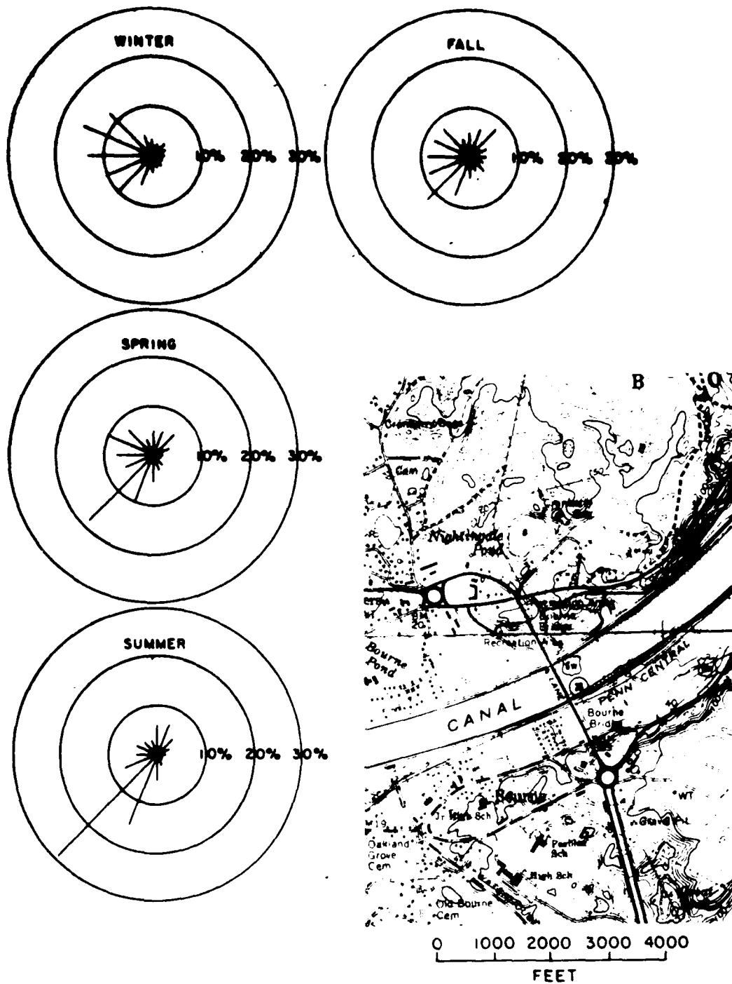
Figure 1. Bourne Bridge and surrounding topographical features, and seasonal wind direction roses. The length of the barb shows the percent of time the wind blew from the indicated direction.
