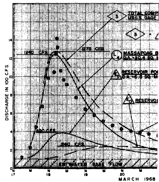
MASSAPOAG BROO USGS. GAGE AT CAN (EAST BRANCH NEPONSE
