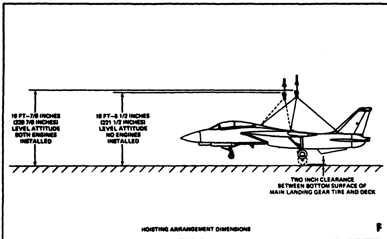
Figure 17. Hoisting
