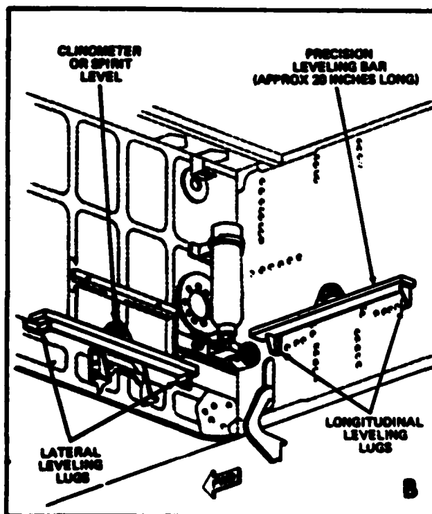
Figure 18. Leveling Points
