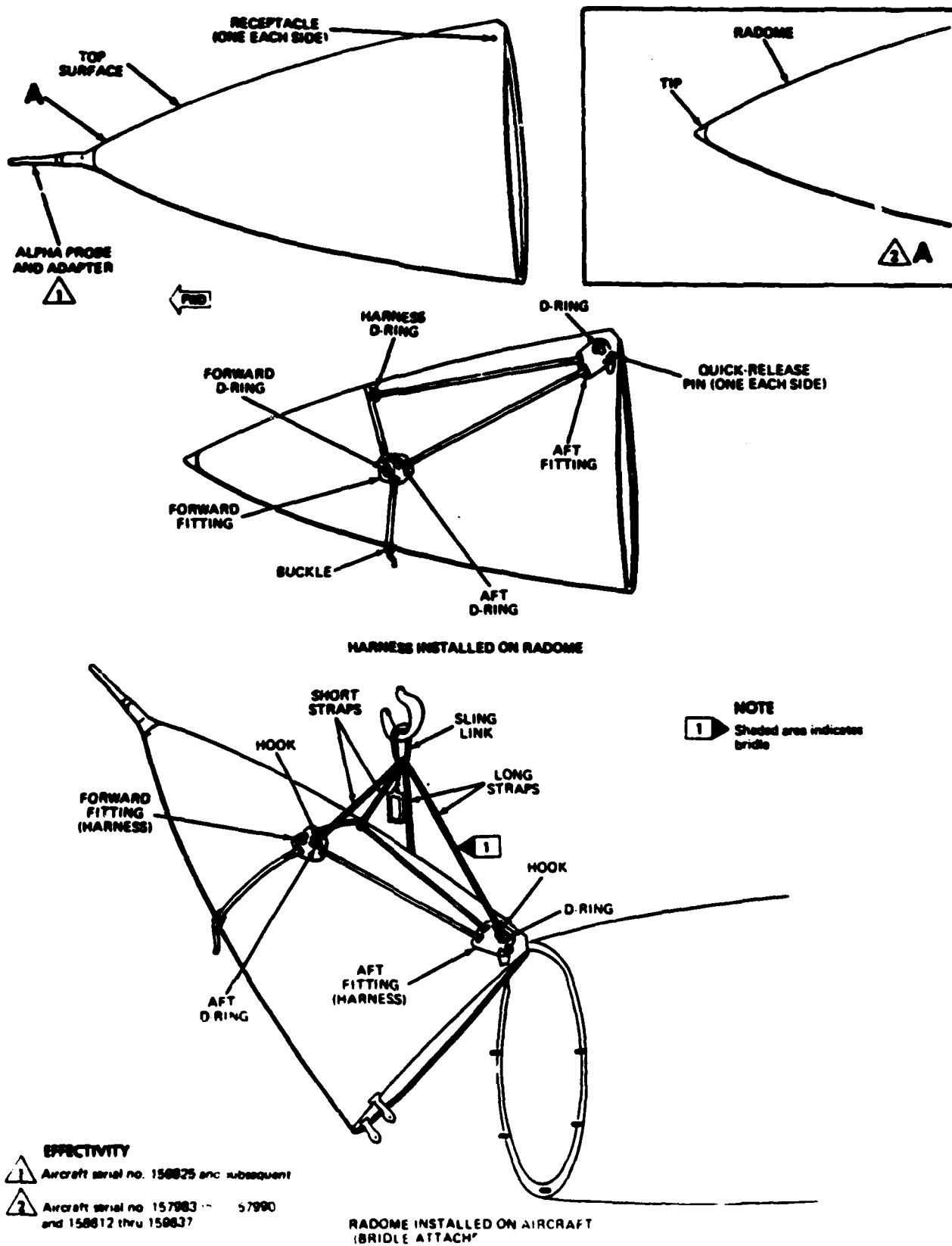
Figure 19. Radome Hoisting
