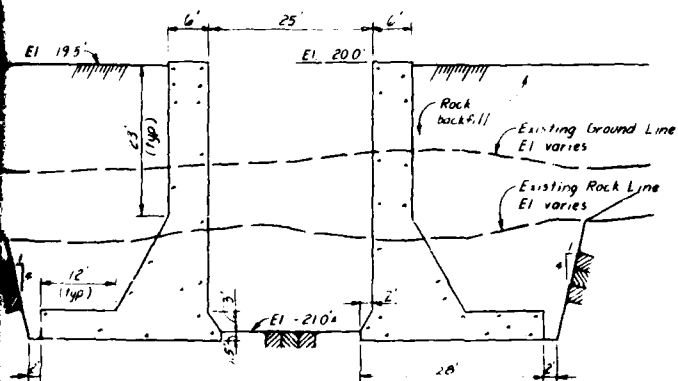
SECTION THRU LOCK CHAMBER
