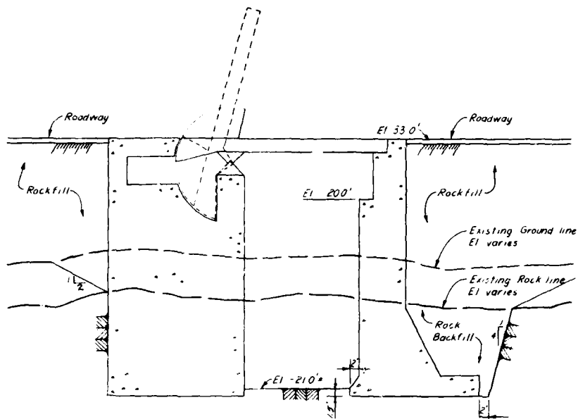
SECTION ON E OF BRIDGE
