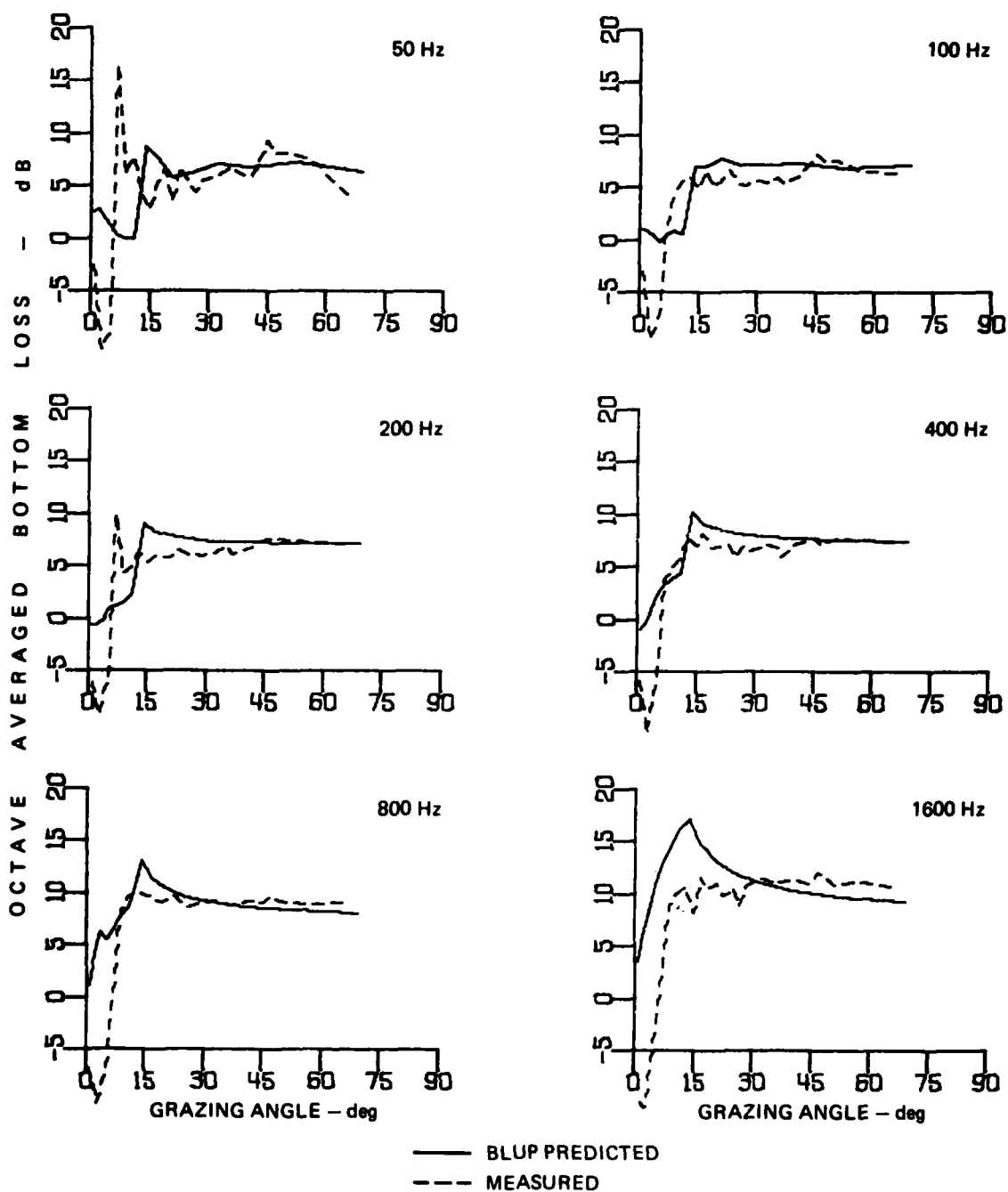
OCTAVE AVERAGED BOTTOM LOSS PREDICTED BY BOTTOM LOSS UPGRADE GEOACOUSTIC PROFILE versus NADC BOTTOM LOSS DATA AT LOCATION 3
