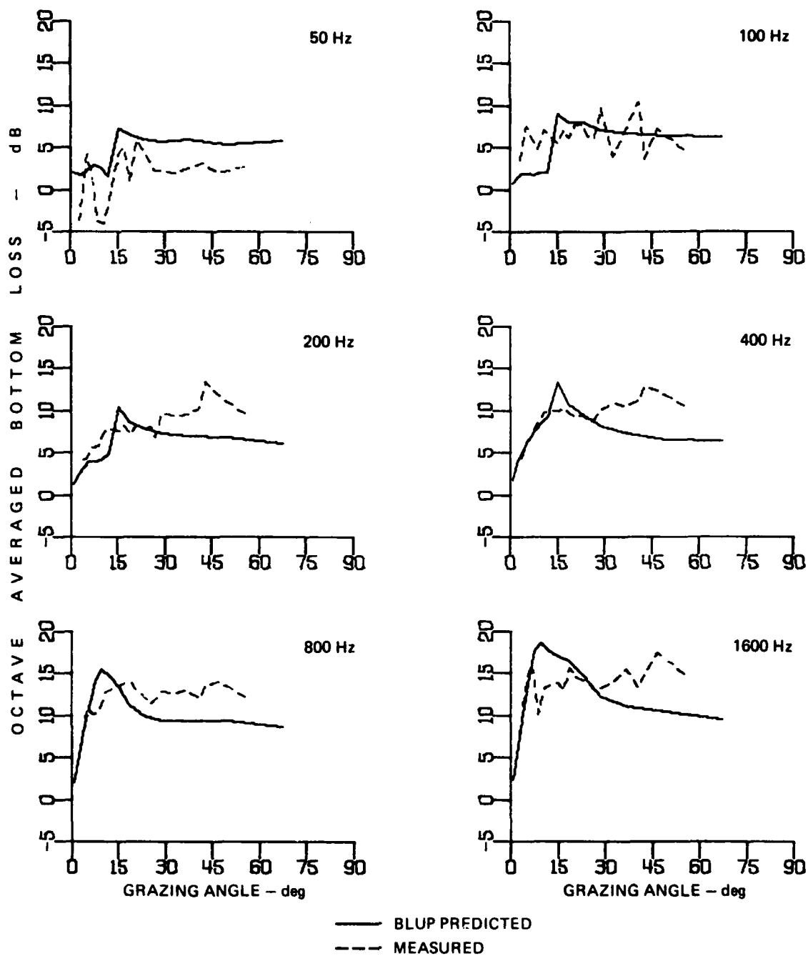
OCTAVE AVERAGED BOTTOM LOSS PREDICTED BY BOTTOM LOSS UPGRADE GEOACOUSTIC PROFILE versus NADC BOTTOM LOSS DATA AT LOCATION 14
