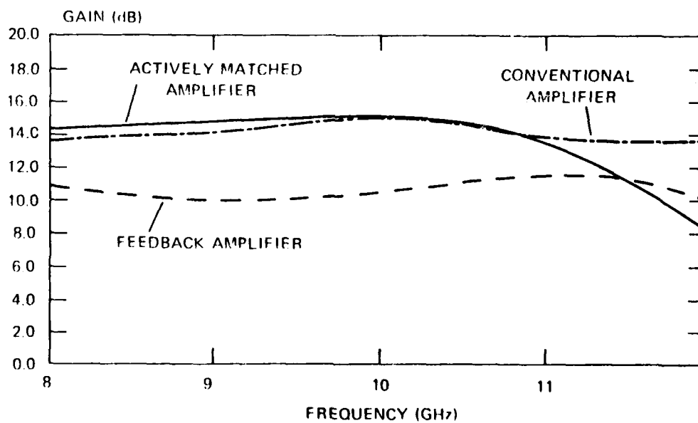
Figure 3-30. Gain Comparison
