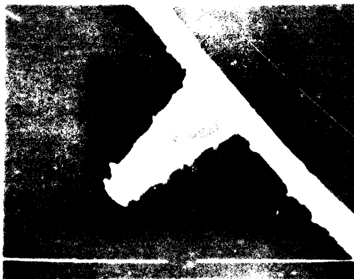
Figure 2-26. Lift-Off Ti-Pt-Au Metallization Patterns Achieved With PMIPK Resist Reveals Wings Less Severe Than With PMMA
