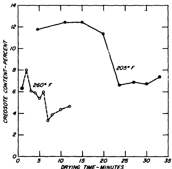
Figure 7.—Effect of drying time and temperature on creosote content of railroad tie particles. (M)151-105
