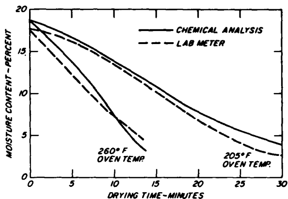
Figure 6.—Moisture content of creosoted railroad tie particles as measured by a laboratory moisture meter and a chemical analysis for creosote and water. (M151-104)
