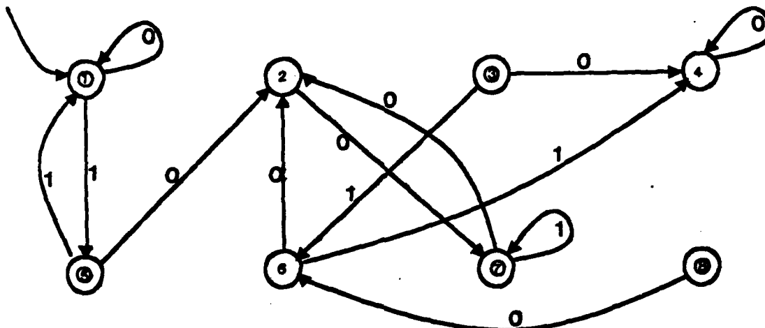
figure 2-4: The results of the other 13 problems
