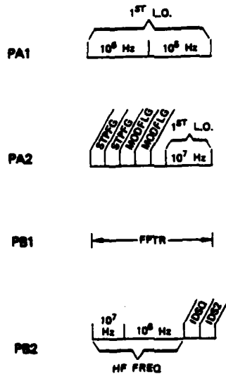
Fig. 14 — \mu P Page Zero Storage Allocation
