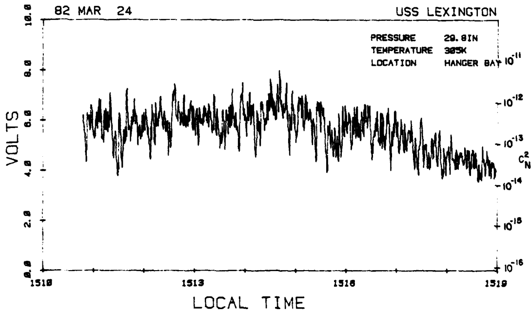
Fig. 12 - Microthermal probe response at forward hanger bay door location from (a) 1453 and (b) 1511 hours on 24 March
