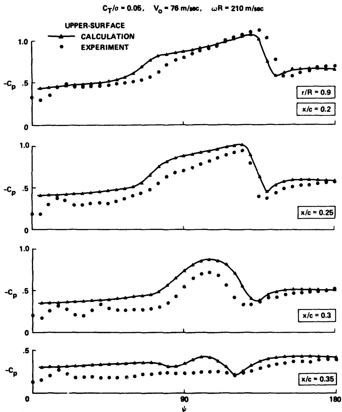
Fig. 9 Comparison of measured and computed pressure coefficient at different chordwise stations, C_T/\sigma = 0.05 , r/R = 0.90 .
