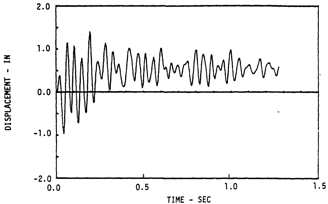
Figure 5.4a. Response of nonlinear system to the force in Figure 5.1a. k_y = 5000
