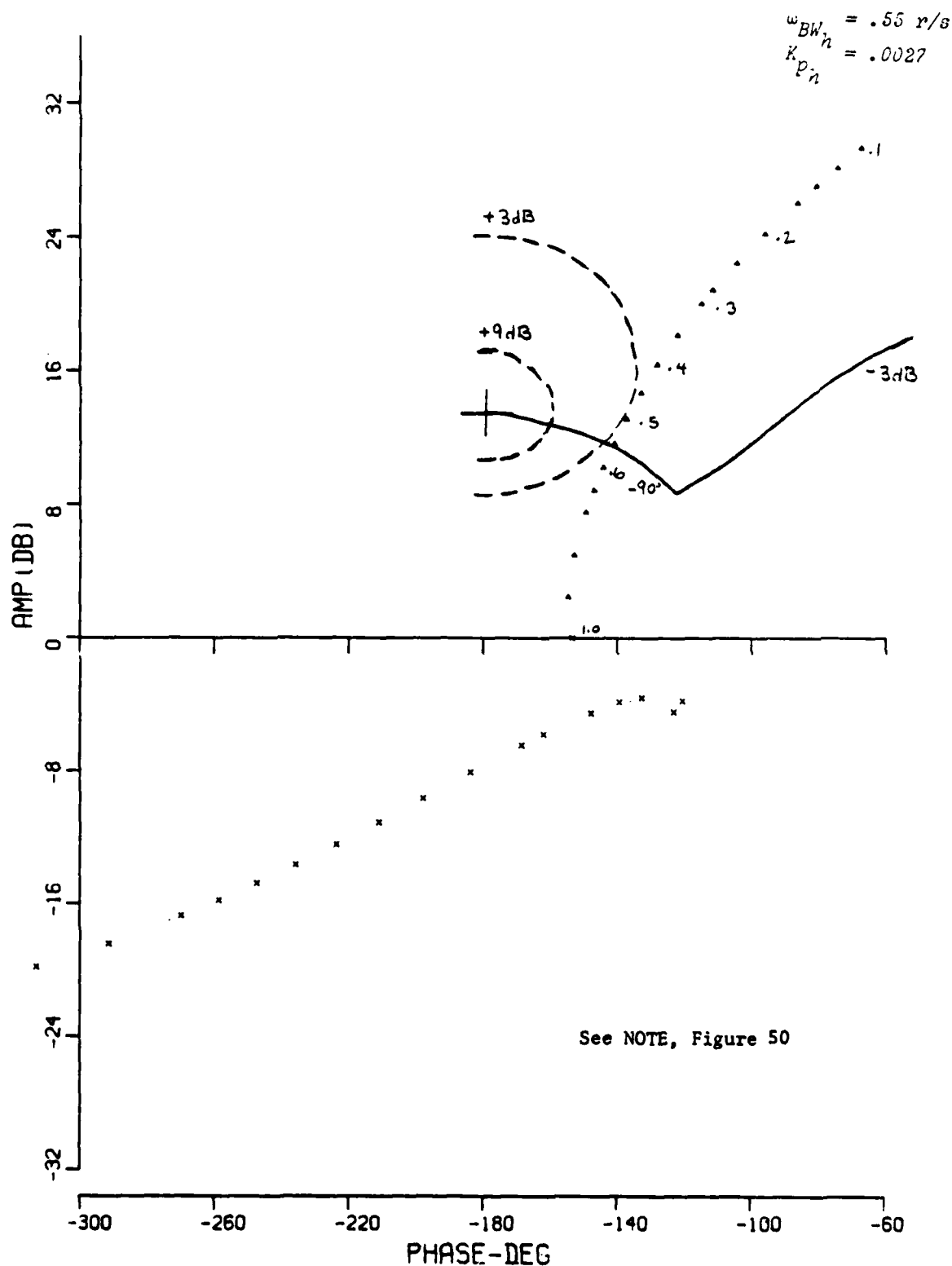
Figure 53. LONG AFT TAIL, HIGH q , X_{MP} = 110' , T_1 = A , h/h_c NICHOLS PLOT
