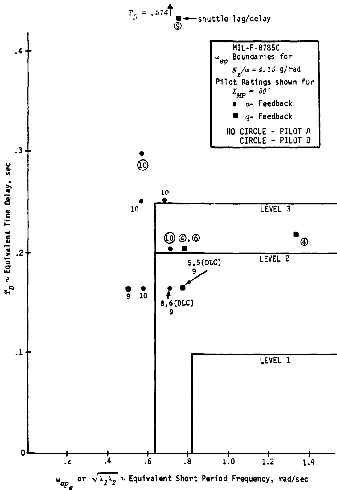
Figure V-A-7. SHORT AFT TAIL CONFIGURATIONS VS ALLOWABLE TIME DELAY
