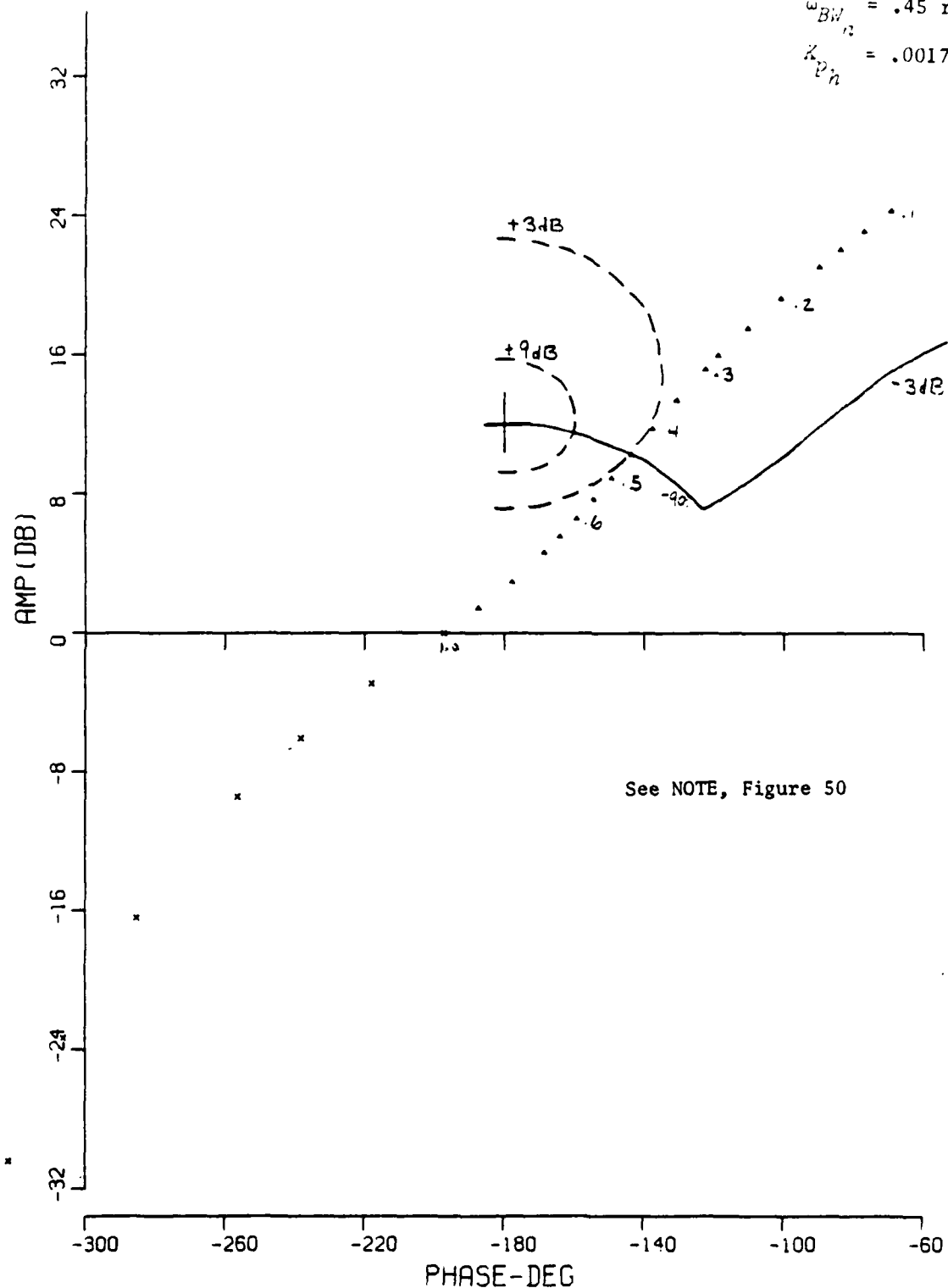
6 MAY 1981 000002 - S-A TQ=1.00 KQ=2.50 HI 1.00 XP=70 DEL=0.00 MULT=LOOP Figure 51. SHORT AFT TAIL, HIGH q , X_{MP} = 70' , T_1 = A , h/h_c NICHOLS PLOT
