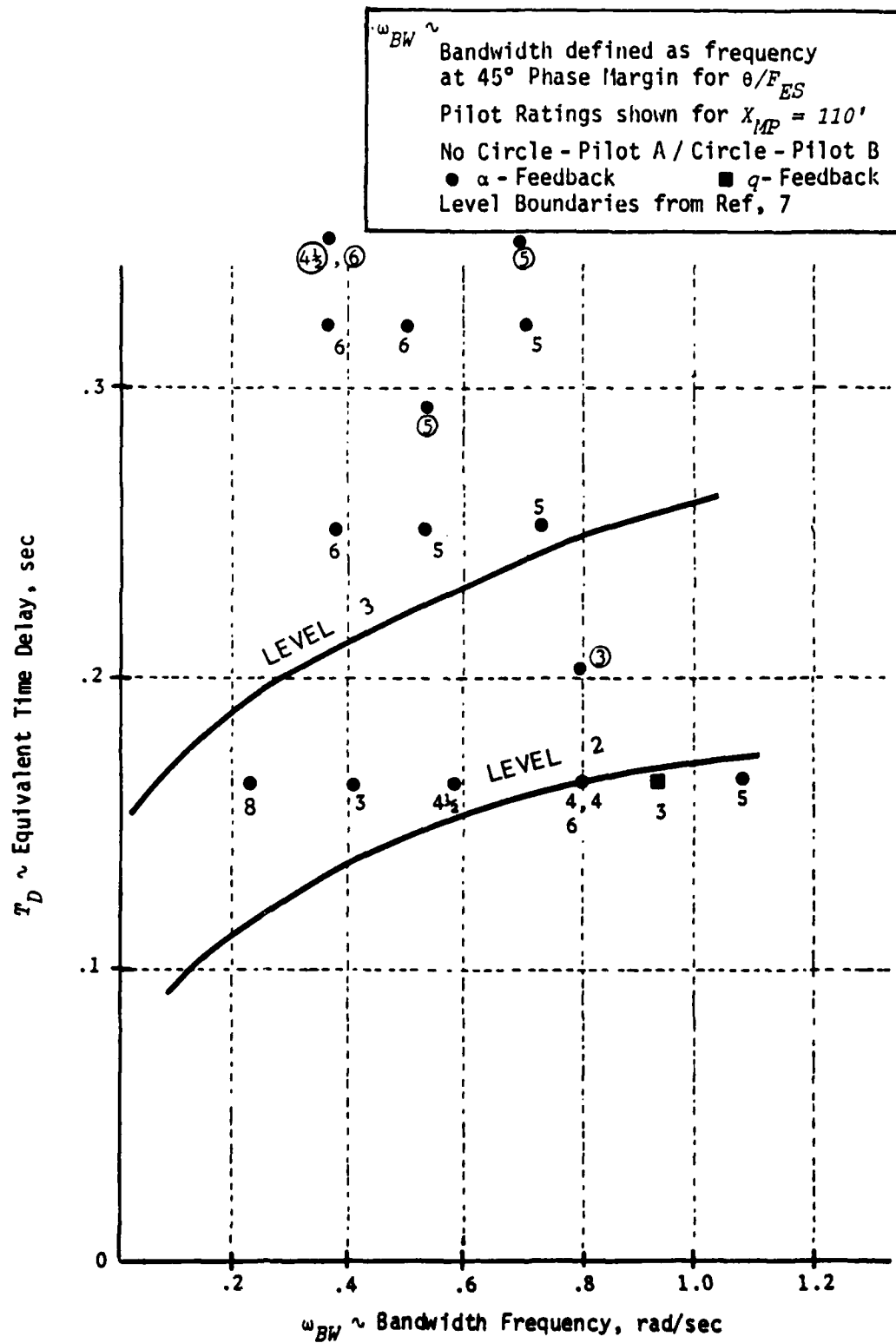
Figure V-C-3. CANARD OPEN LOOP \theta/F_{ES} BANDWIDTH VS TIME DELAY
