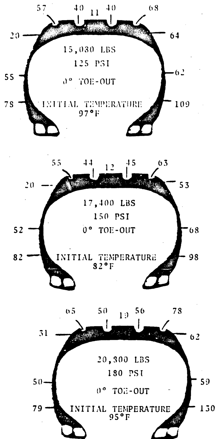
Figure 10. Taxi Test Tire Surface Temperature Rise at 0° Toe-Out
