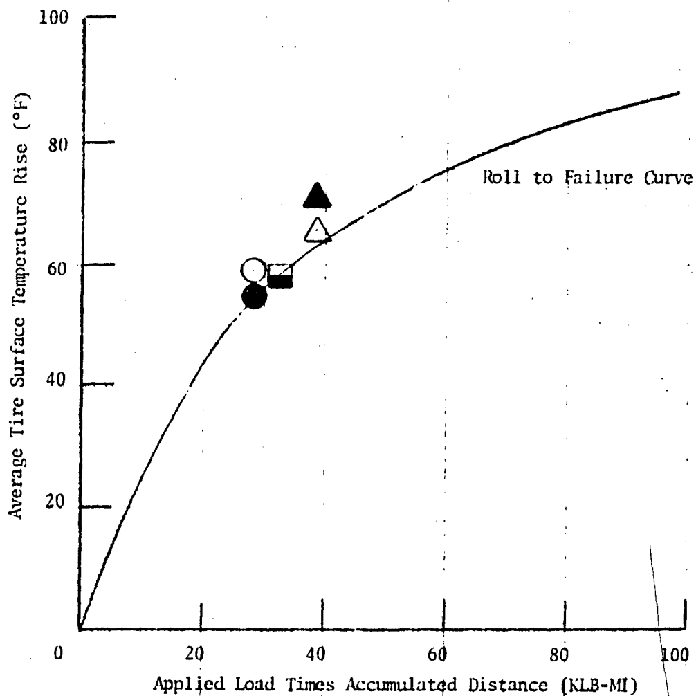
Figure 27. Average Tire Surface Temperature Rise Versus Applied Load Times Accumulated Distance Comparison Between Laboratory Roll to Failure Test and Taxi Tests for TIRE A
