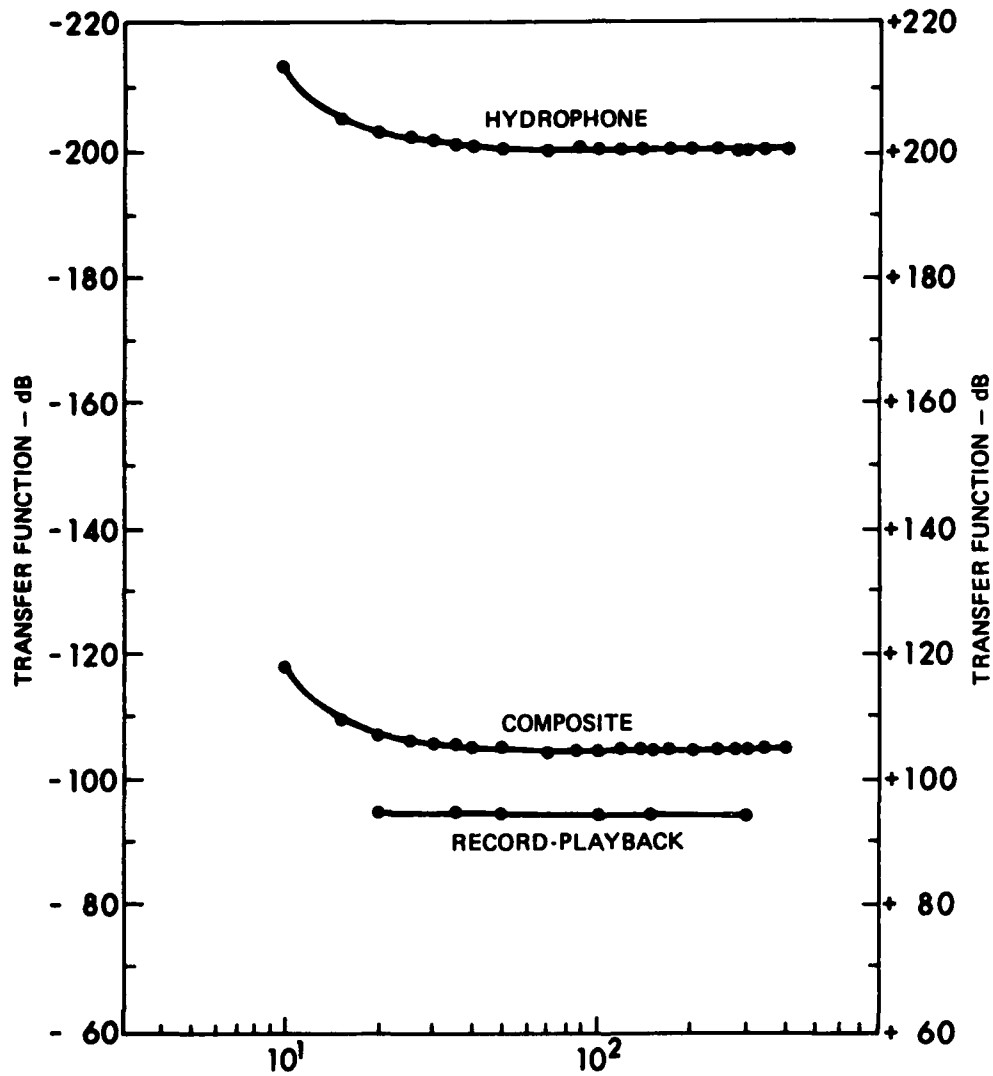
FIGURE 4 TRANSFER FUNCTIONS FOR HYDROPHONE 4 HYDROPHONE TRANSFER FUNCTION (V/ \mu Pa) AND RECORD-PLAYBACK TRANSFER FUNCTION (V/DIGITIZED NUMERIC VALUE) USE THE LEFT SCALE. THE COMPOSITE TRANSFER FUNCTION ( \mu Pa/DIGITIZED NUMERIC VALUE) USES THE RIGHT SCALE.
