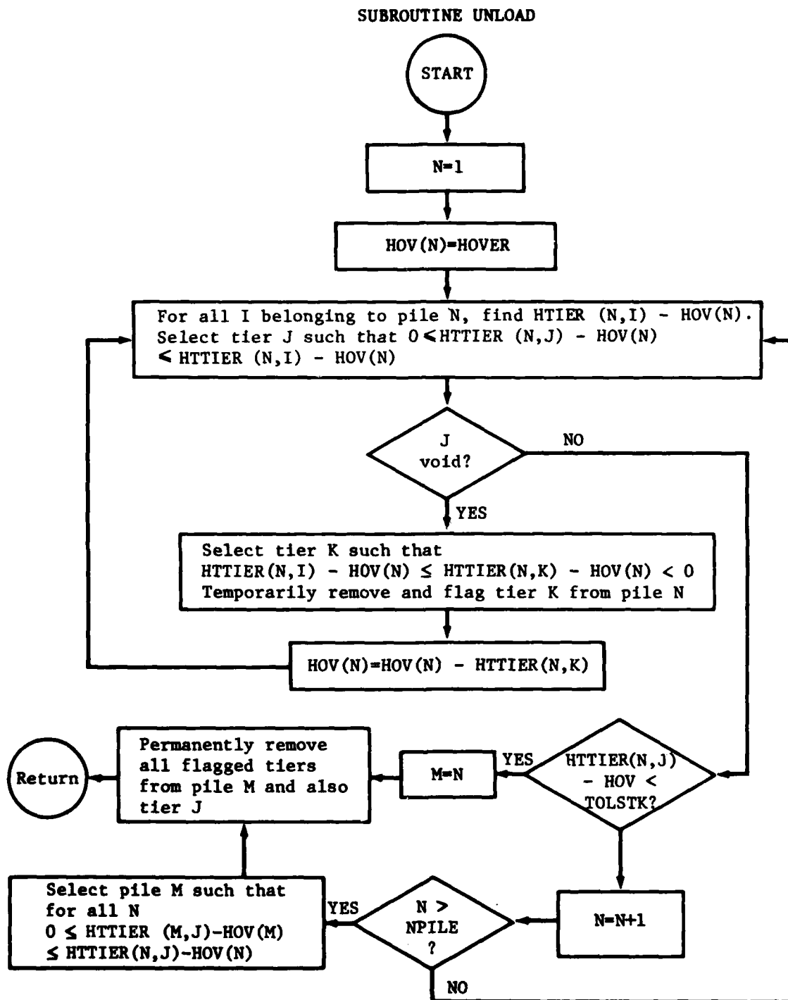
Figure 28 - Subroutine UNLOAD, Flowchart
