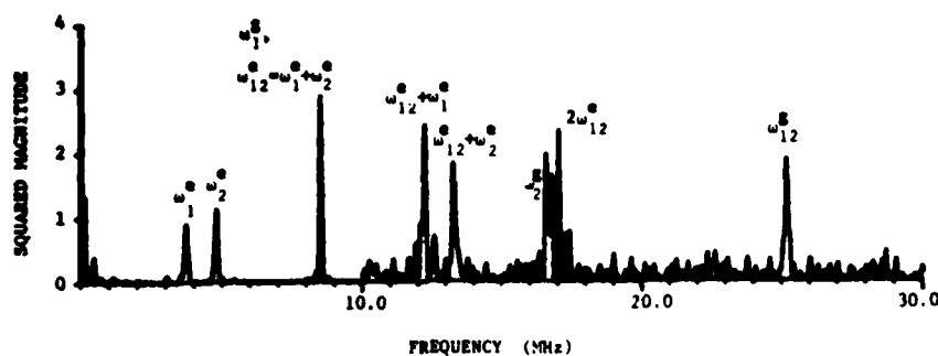
FIG. 2. Squared magnitude of the Fourier transform of the data in Fig. 1. The data were first multiplied by \exp(\tau/1.2\ \mu\text{sec}) . The vertical scale is 100 times more sensitive for frequencies beyond 10 MHz.
