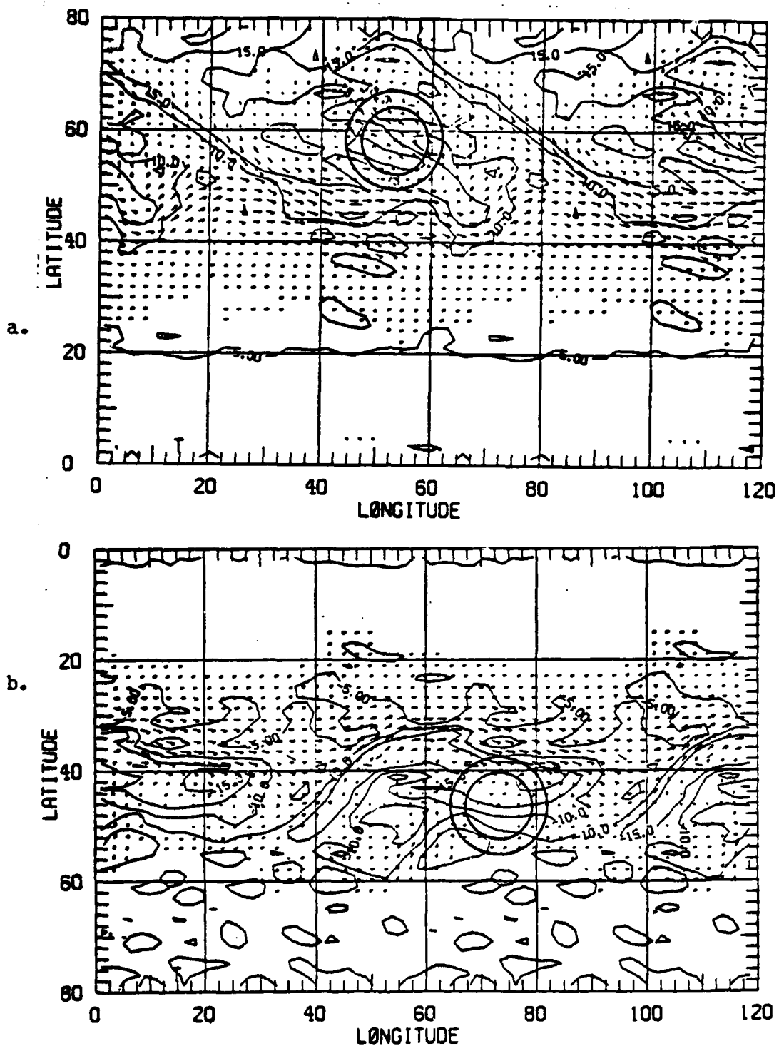
Figure 19. Same as Fig. 13 except for initial time + 168 hours.
