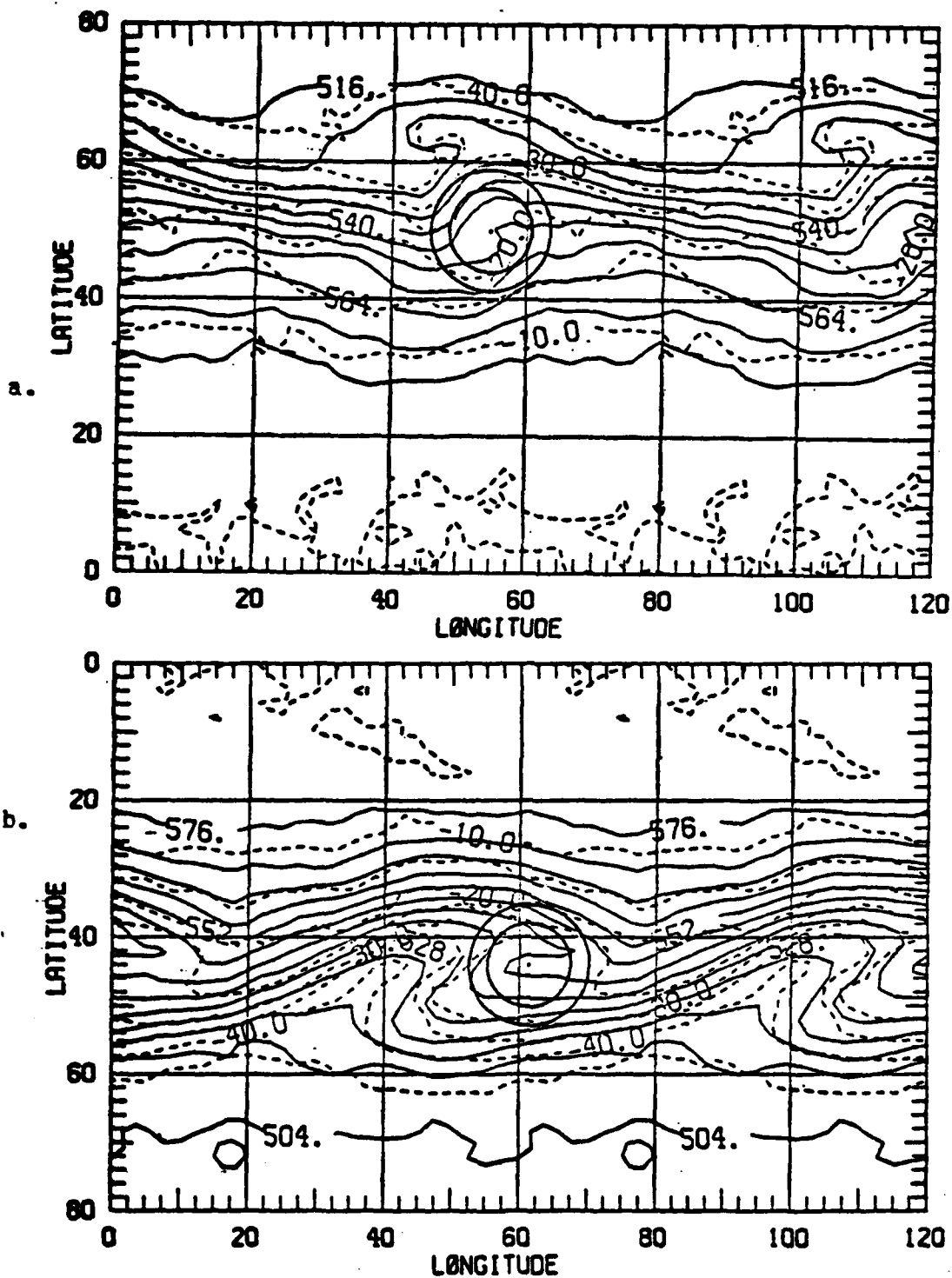
Figure 16. Same as Fig. 12 except for initial time + 144 hours.
