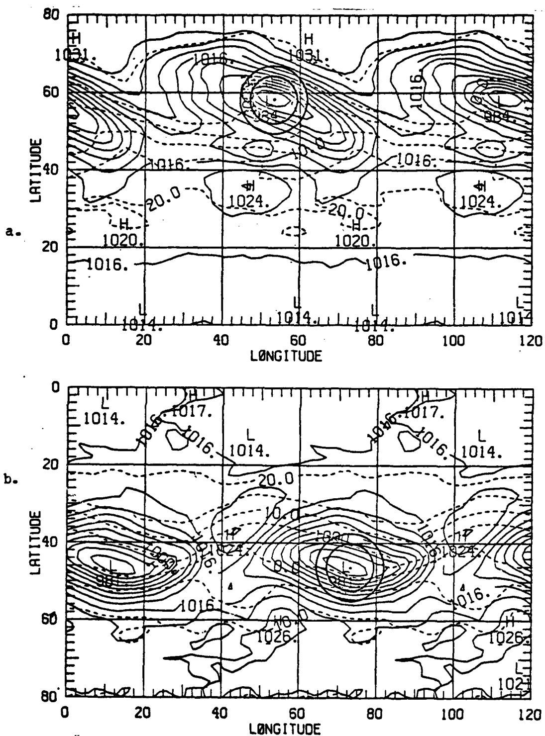
Figure 10. Same as Fig. 4 except for initial time + 168 hours.
