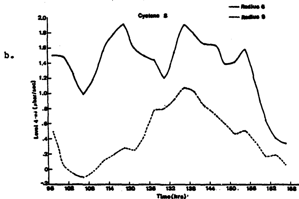
Figure 36. Model vertical velocity for level 4. (- μ bar sec -1 ) a. and b. as in Fig. 30.
