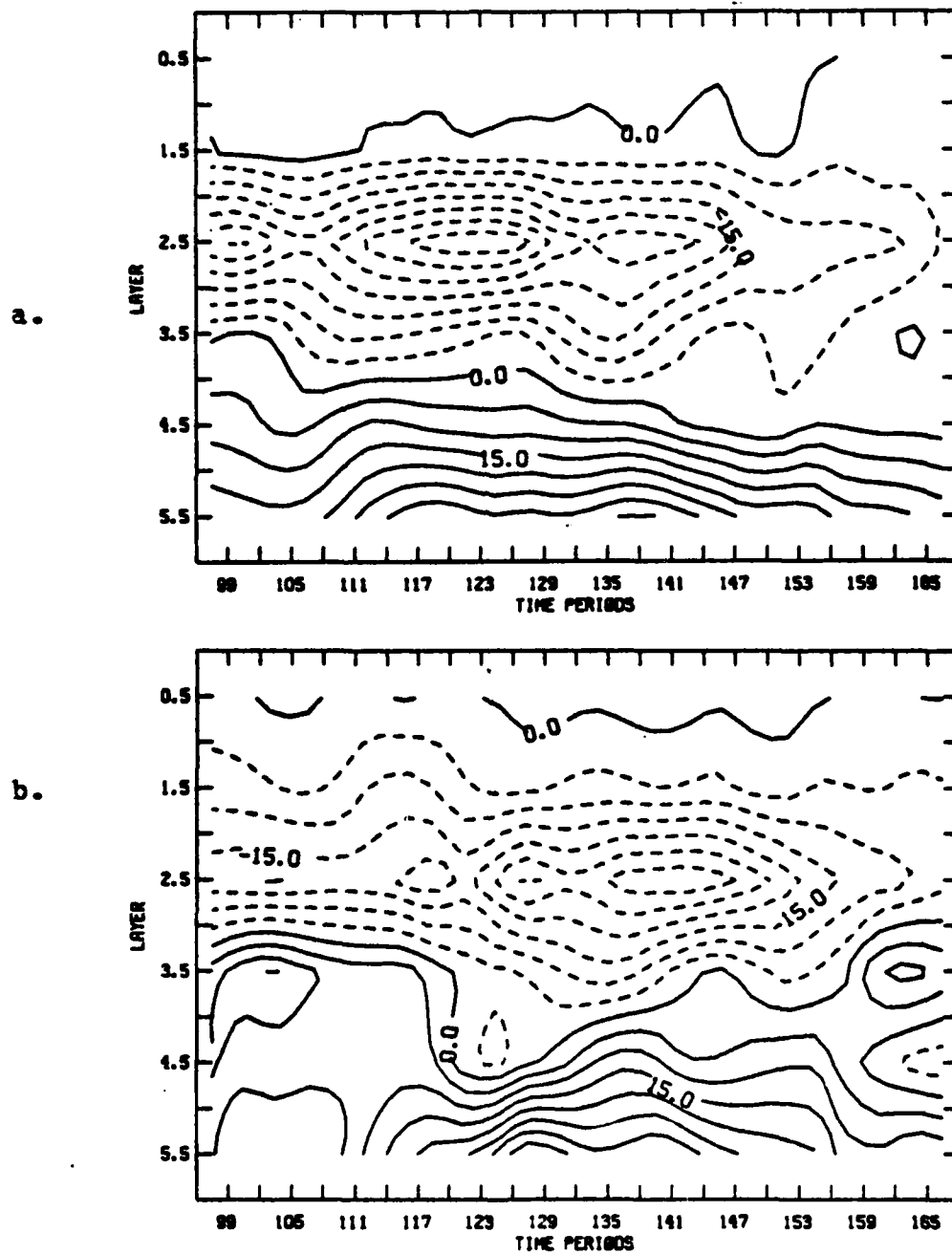
Figure 33. Cyclone S lateral mass transport time section. ( \times 10^{12} g sec ^{-1} ) a. and b. as in Fig. 28.
