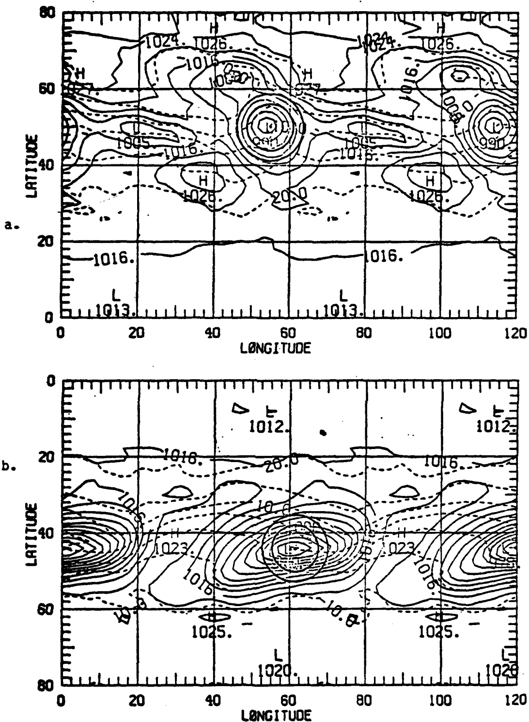
Figure 8. Same as Fig. 4 except for initial time + 144 hours.
