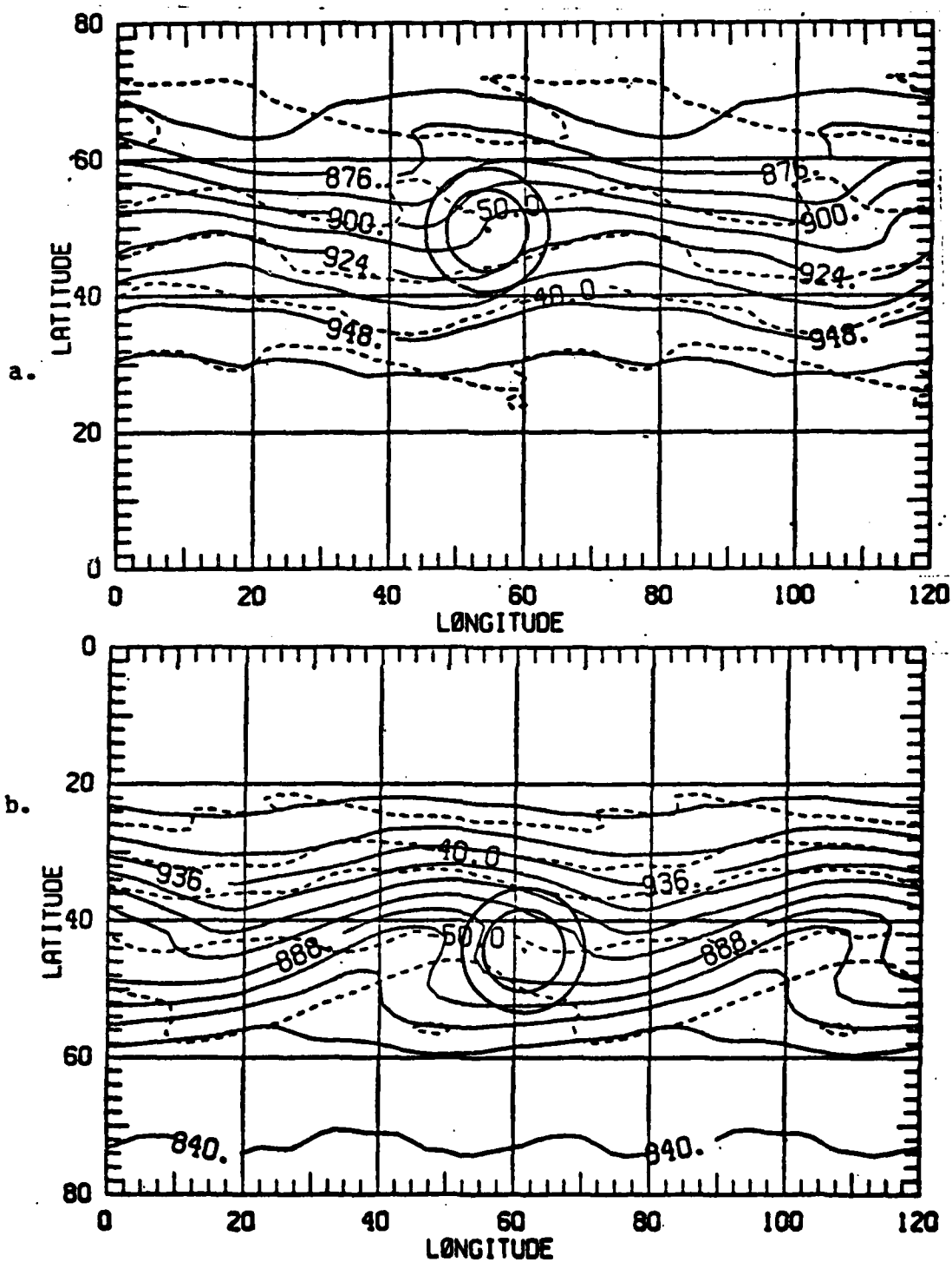
Figure 24. Same as Fig. 20 except for initial time + 144 hours.
