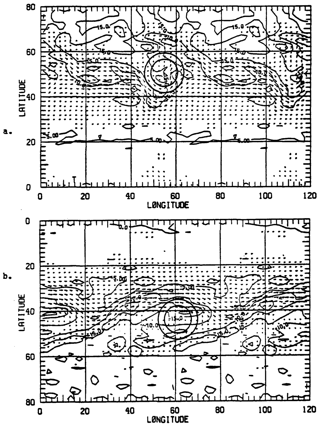
Figure 17. Same as Fig. 13 except for initial time + 144 hours.
