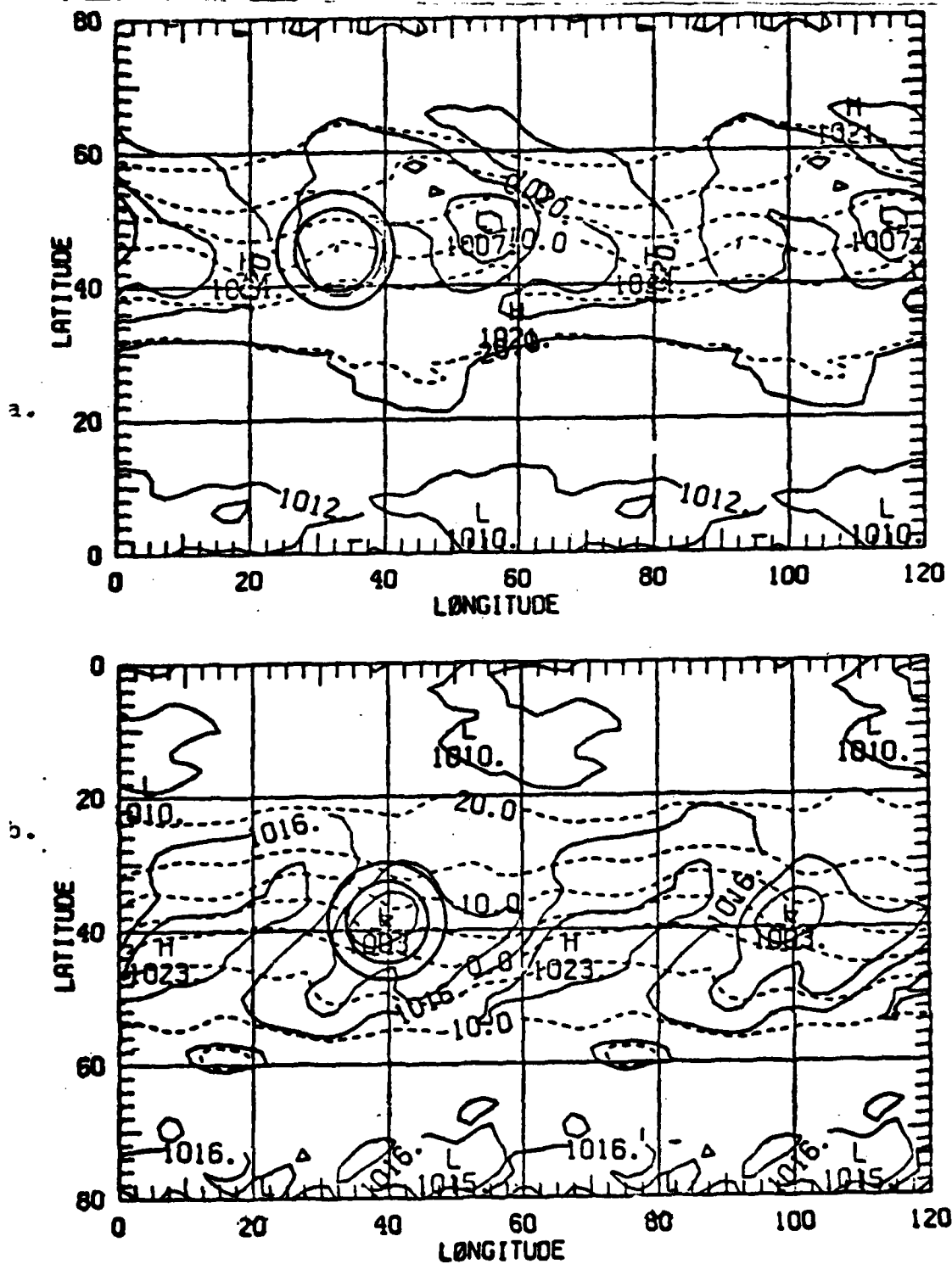
Figure 4. Surface pressure and temperature fields valid at initial time + 96 hours. Isobars (solid) are in millibars. Isotherms (dashed) are in °C. a. and b. as in Fig. 3.
