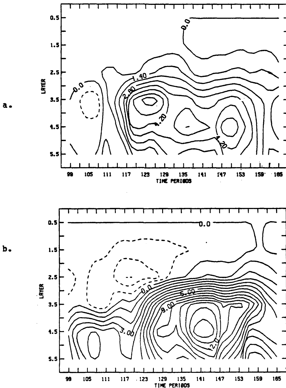
Figure 39. Budget vertical velocity error time section for cyclone N1. Model vertical velocities minus budget vertical velocities. ( -\mu bar \text{sec}^{-1} ) a. and b. as in Fig. 28.
