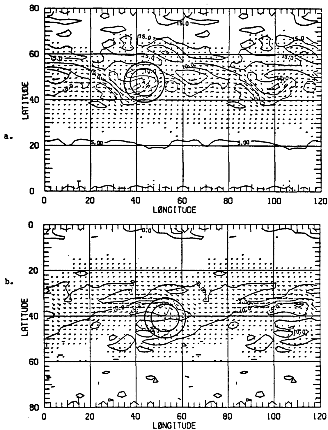
Figure 15. Same as Fig. 13 except for initial time + 120 hours.
