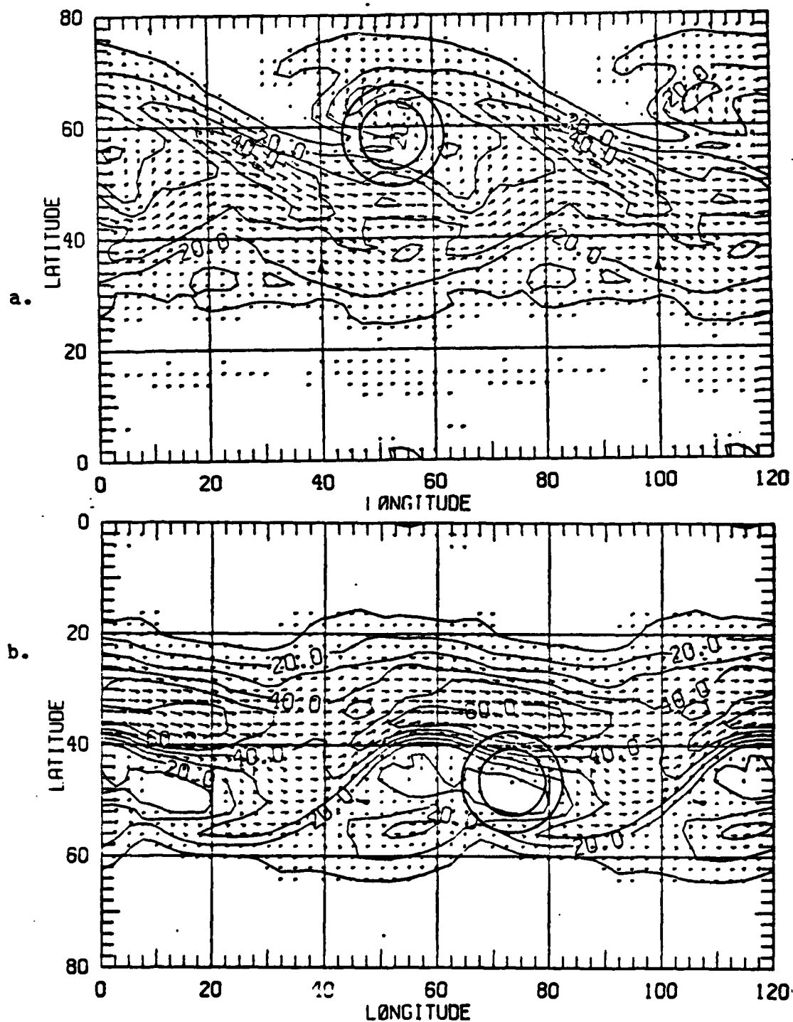
Figure 27. Same as Fig. 21 except for initial time + 168 hours.
