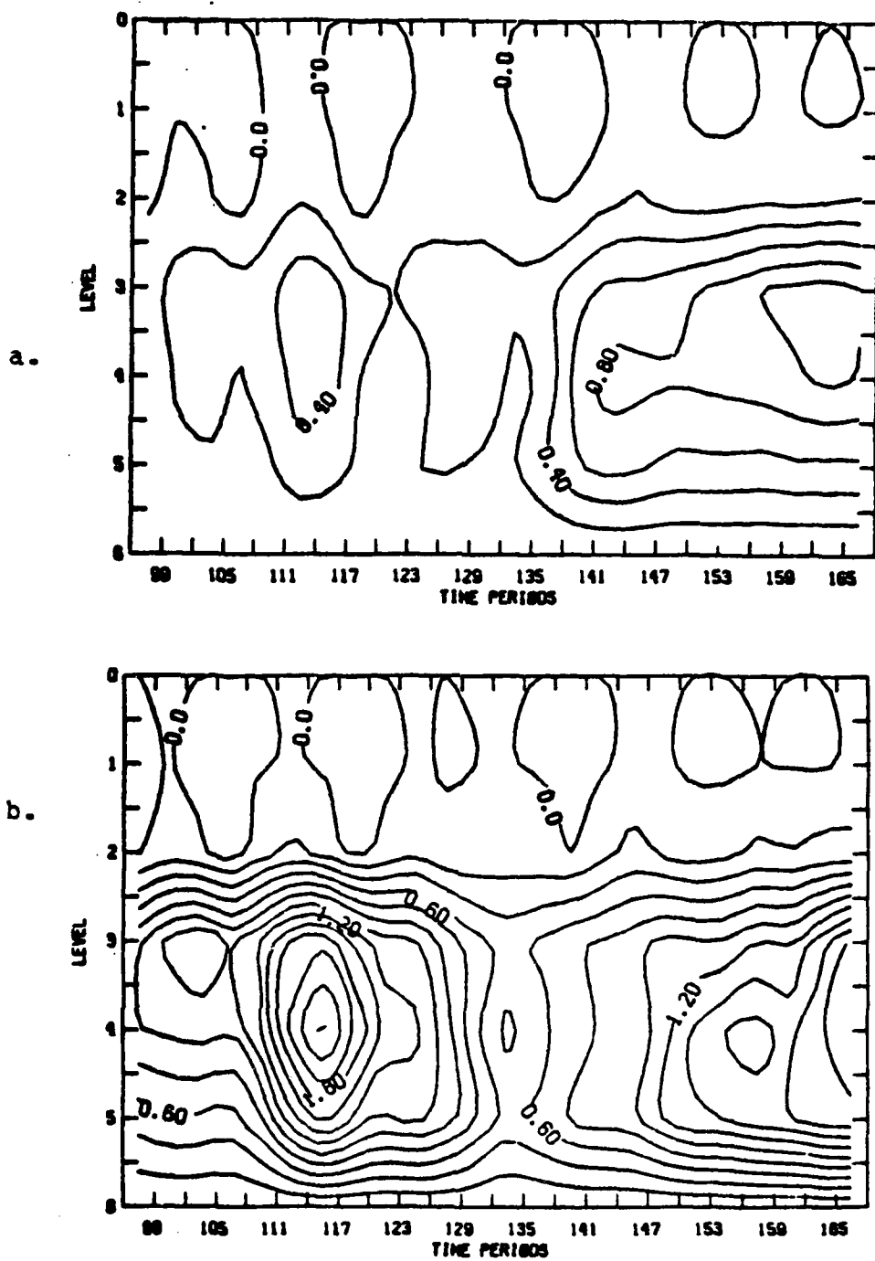
Figure 34. Cyclone N1 model vertical velocity time section. ( \mu bar \text{sec}^{-1} ) a. and b. as in Fig. 28.
