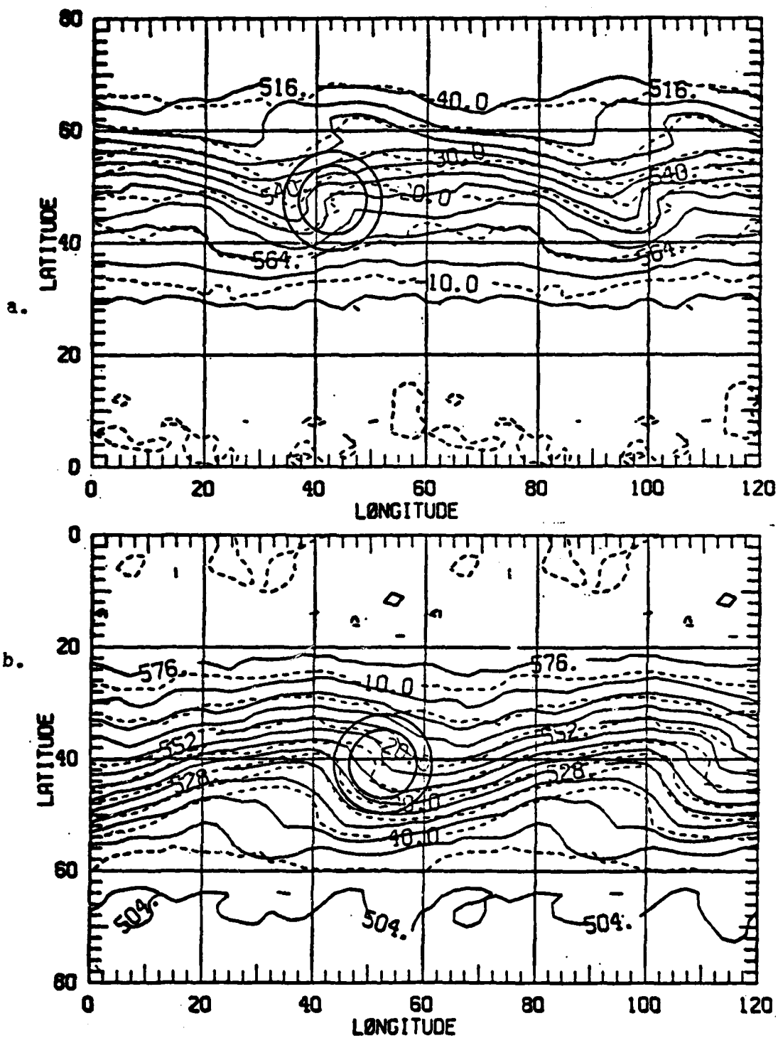
Figure 14. Same as Fig. 12 except for initial time + 120 hours.
