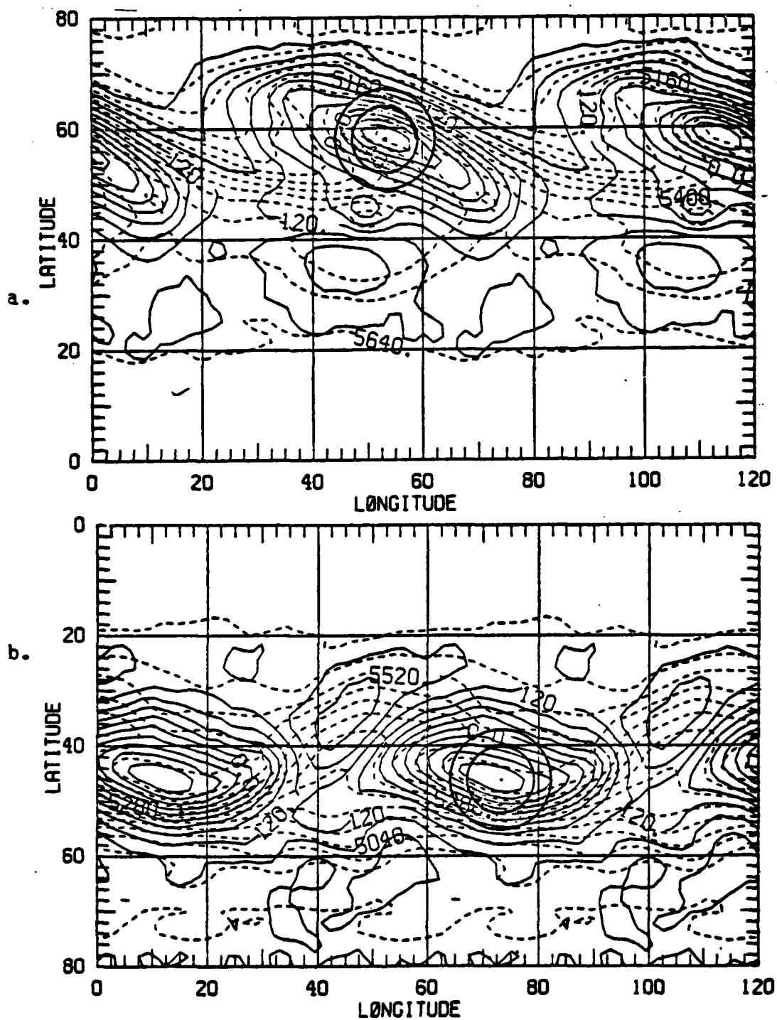
Figure 11. Same as Fig. 5 except for initial time + 168 hours.
