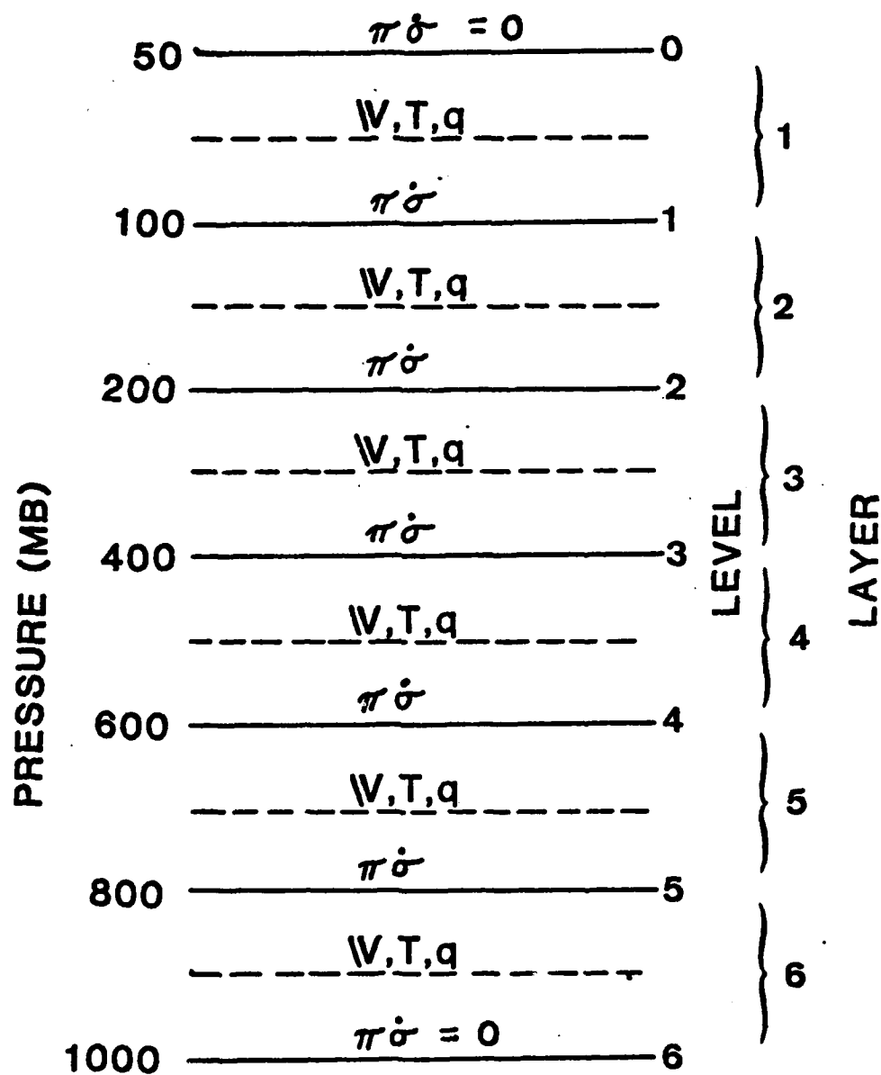
Figure 1. Vertical distribution of model large-scale prognostic variables. Pressure values of sigma levels vary with the surface pressure. A surface value of 1000 mb is assumed in this figure. (After Sandgathe, 1981)
