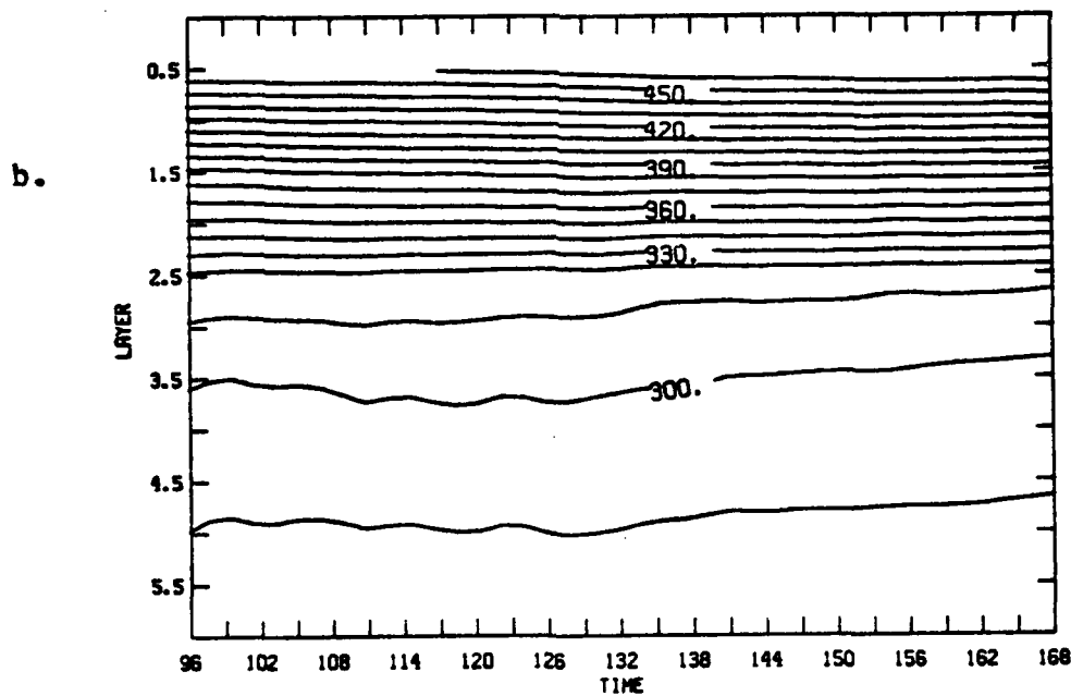
Figure 29. Cyclone S area-averaged potential temperature time section. ( ^{\circ}\text{K} ) a. and b. as in Fig. 28.
