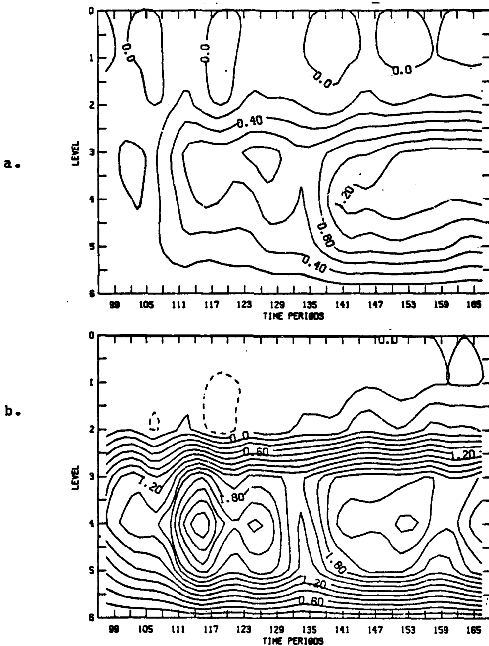
Figure 37. Mass budget vertical velocity time section for cyclone #1. ( -\mu\text{bar sec}^{-1} ) a. and b. as in Fig. 28.
