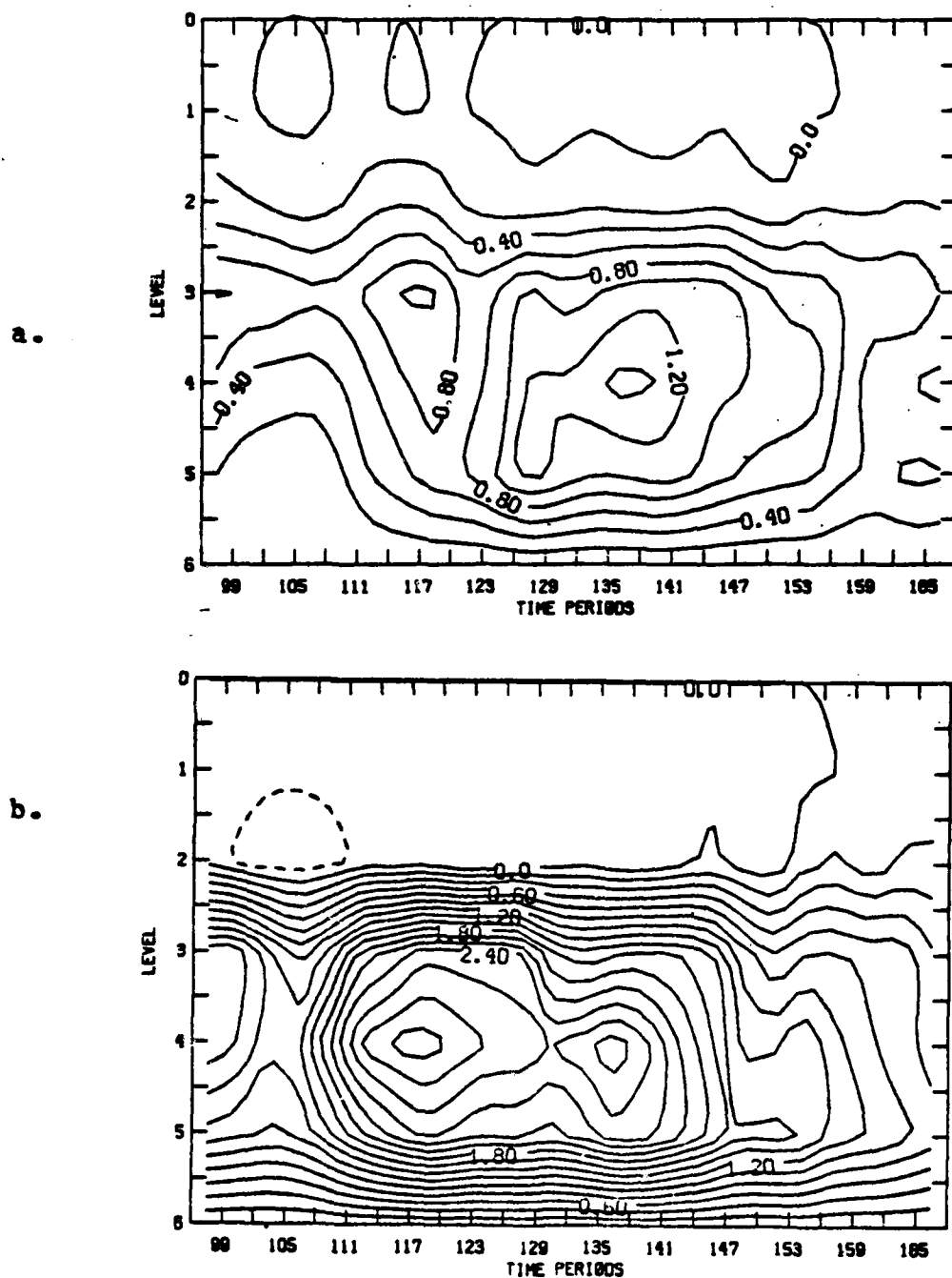
Figure 38. Mass budget vertical velocity time section for cyclone S. ( \mu\text{bar sec}^{-1} ) a. and b. as in Fig. 28.
