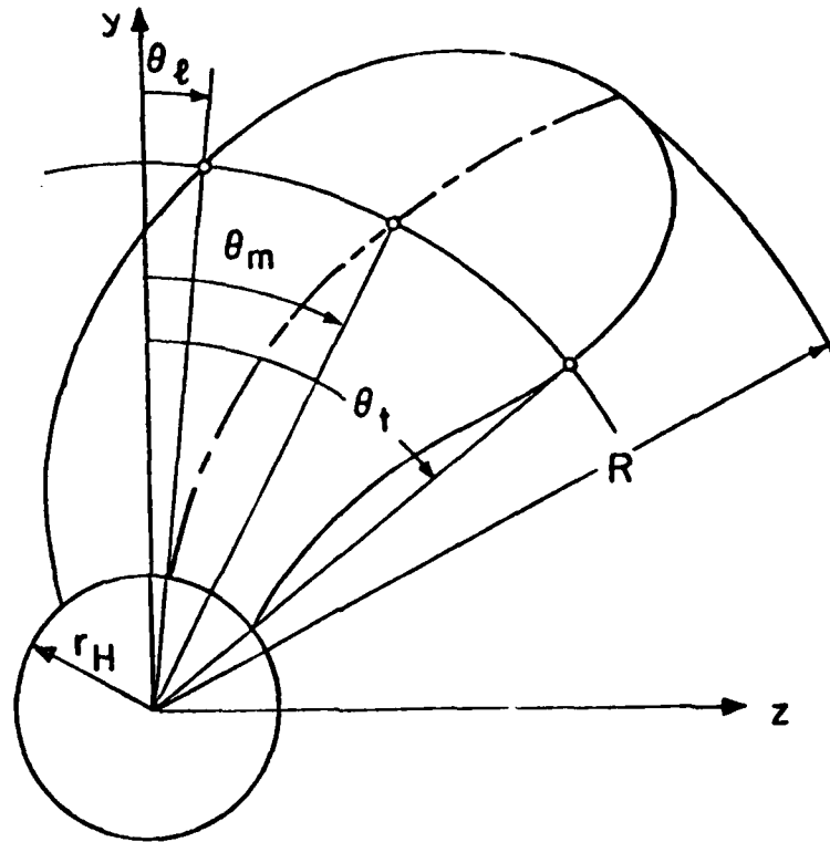
Figure 3.1.1 - Projected view of blade looking downstream
