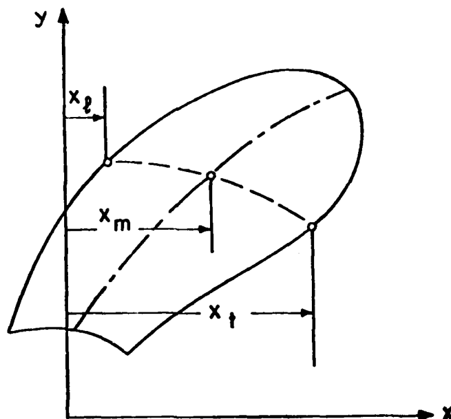
Figure 3.1.1 - Projected view of blade looking downstream
