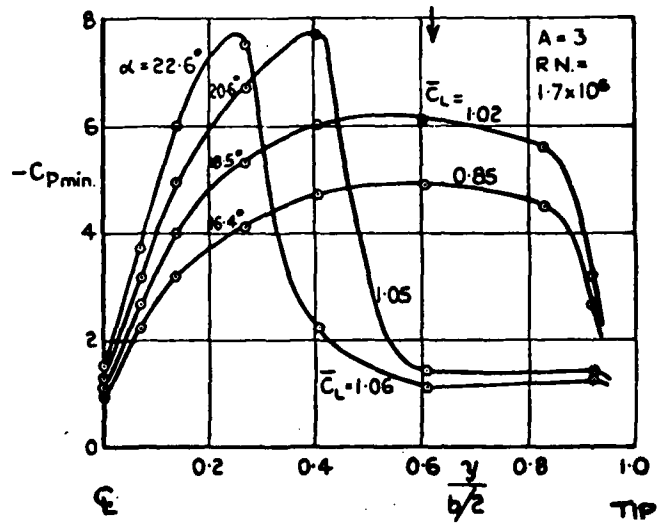
FIG. 4.1.9a MINIMUM PRESSURE NEAR LEADING EDGE ON 45° SWEEP-BACK WING vs. FRACTION OF SEMI-SPAN
