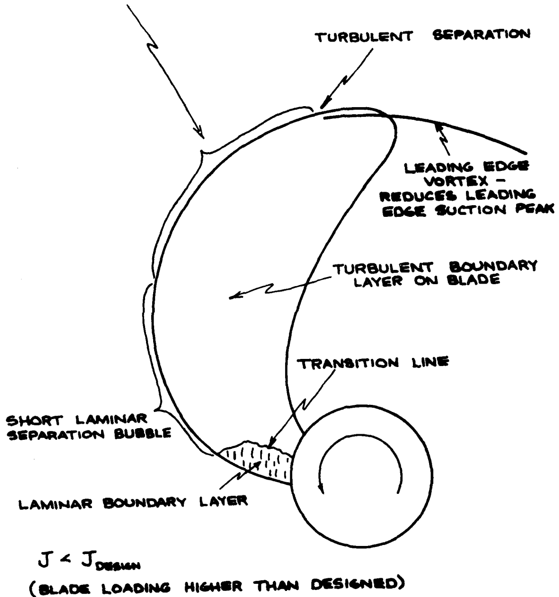
Figure 6.3.3 - Schematic of suction side flow on full-scale propeller blade
