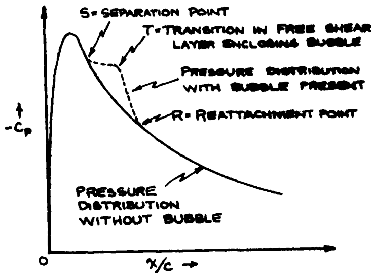
FIG. C.2.4a SCHEMATIC OF UPPER SURFACE PRESSURE DISTRIBUTION ON FOIL WITH SHORT BUBBLE
