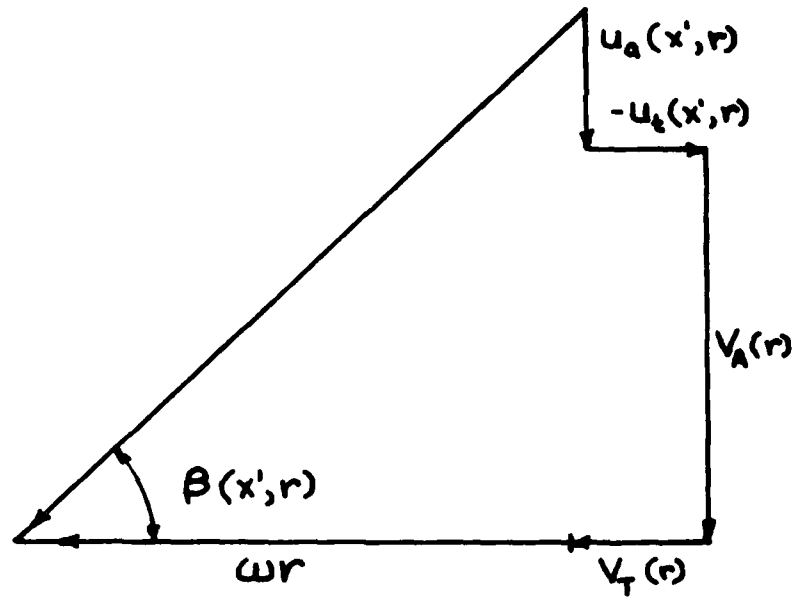
Figure B.2.1 - Velocity diagram in transition wake
