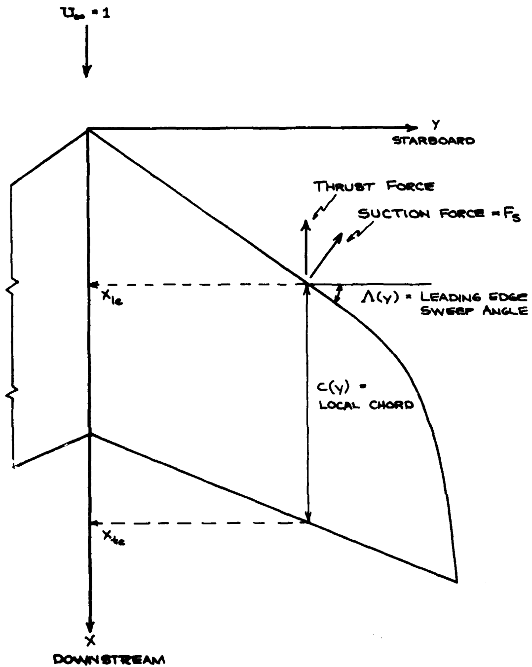
Figure A.3.1 - Plan view of swept wing
