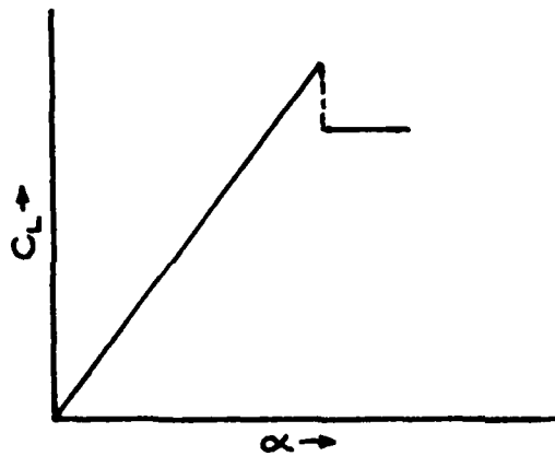
b) Leading edge stall (moderately thick sections)
