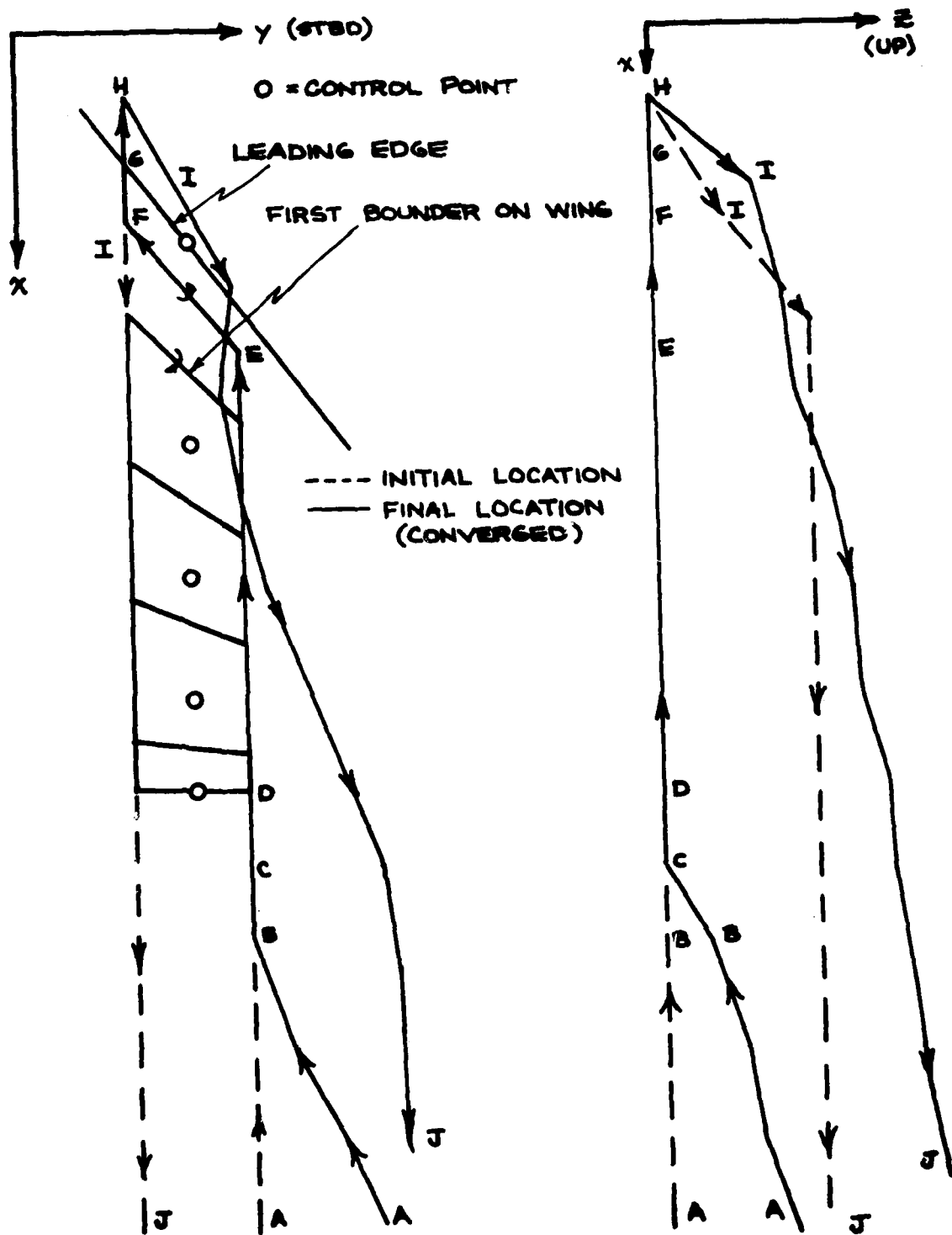
Figure 5.2.4 - Typical leading edge horseshoe vortex in Mehrotra & Lan model
