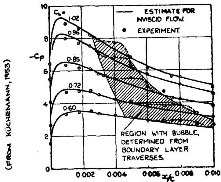
FIG. C.2.4b PRESSURE DISTRIBUTION NEAR NOSE OF NACA 63-009 SECTION
