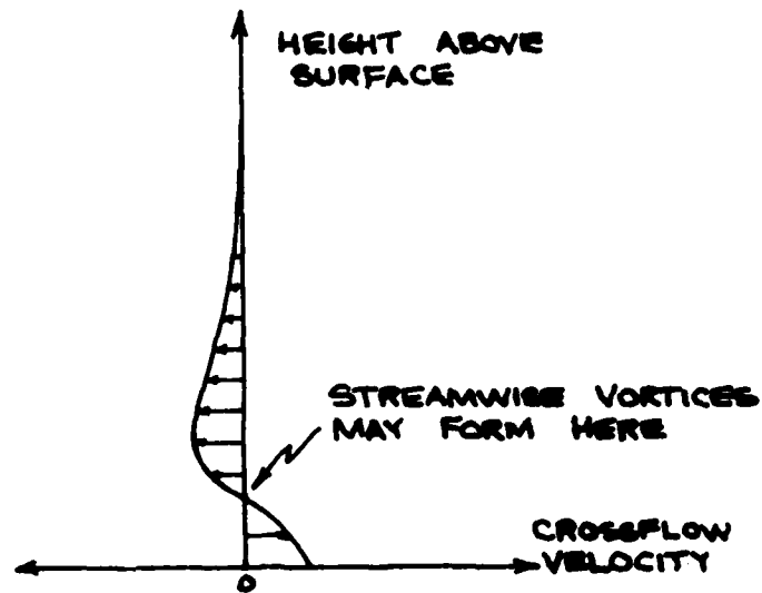
CROSSFLOW VELOCITY AT SECTION A-A
