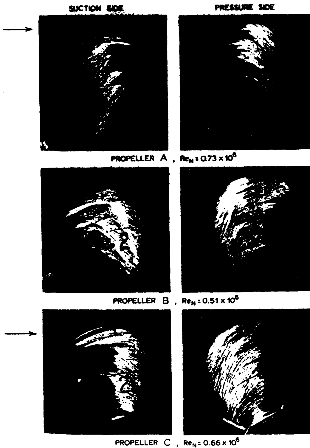
Figure 4.1.7 - Paint flow patterns on 3 propellers at 30% slip
