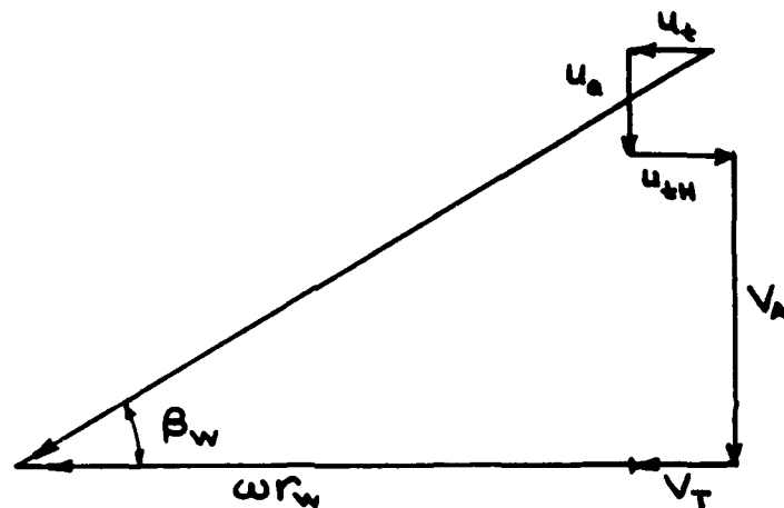
Figure B.1.1 - Velocity diagram at ultimate tip vortex
