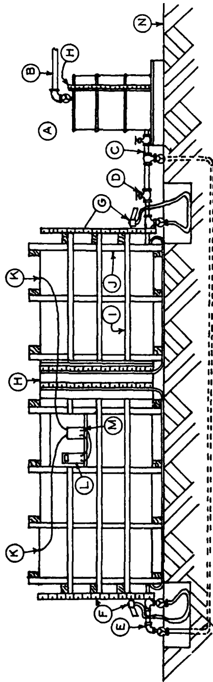
Figure 1. Box model
