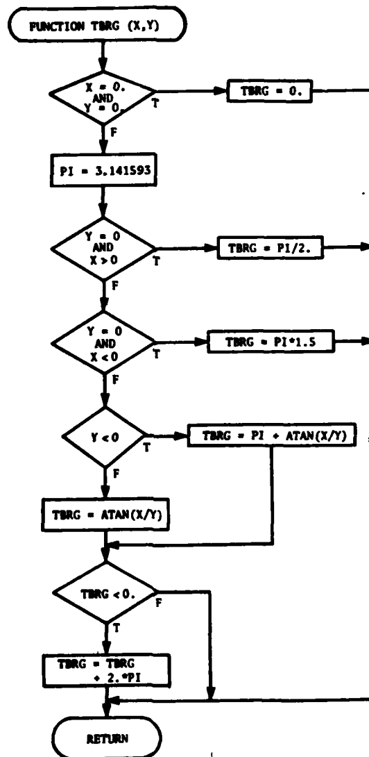
Figure 9-5. Function TBRG
