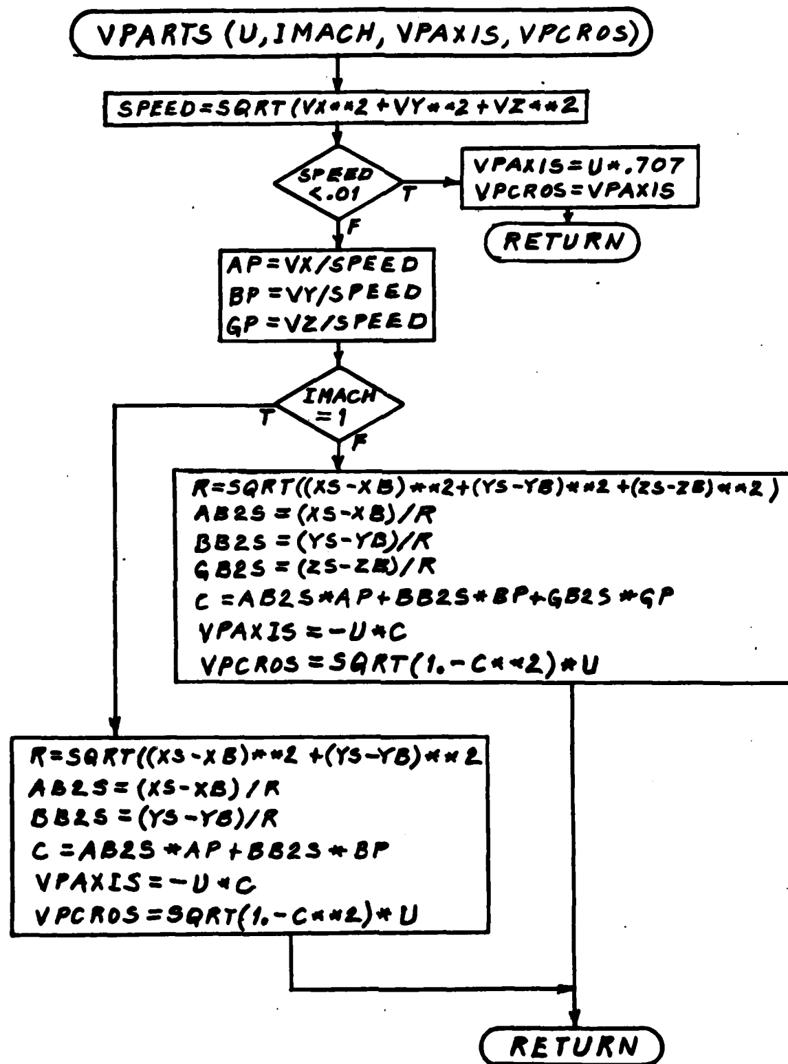
Figure 11-7. Subroutine VPARTS
