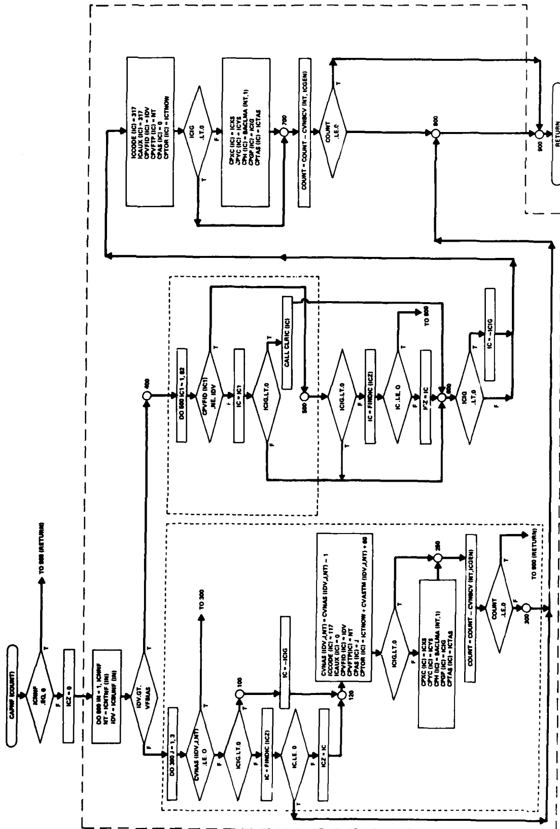
Figure 6-20. Subroutine CAPNF
