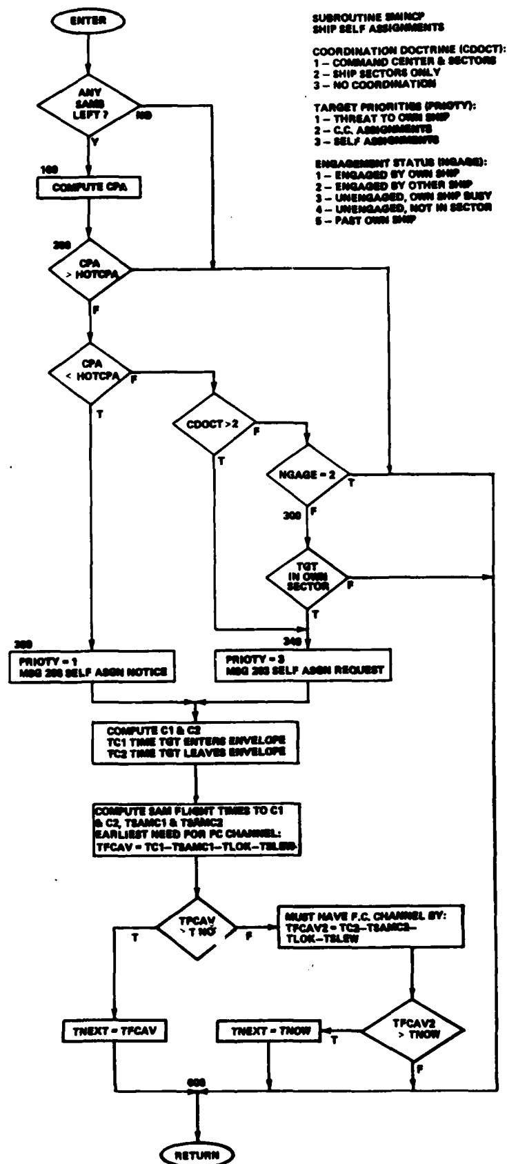
Figure 9-7. Subroutine SMINCP
