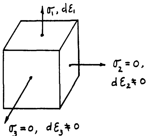
Figure 2A. Stresses and Incremental Plastic Strains for Uniaxial Tension
