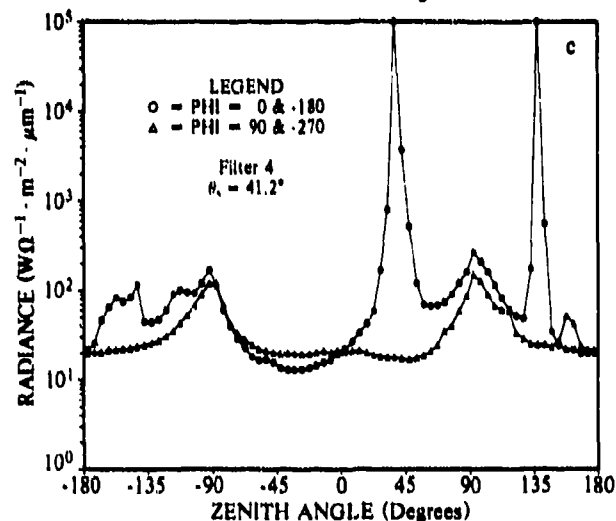
Fig. 3-10. Flight C-379 (Rodby, Denmark), Clear Sky over Ocean with Glitter, 6000m AGL.
