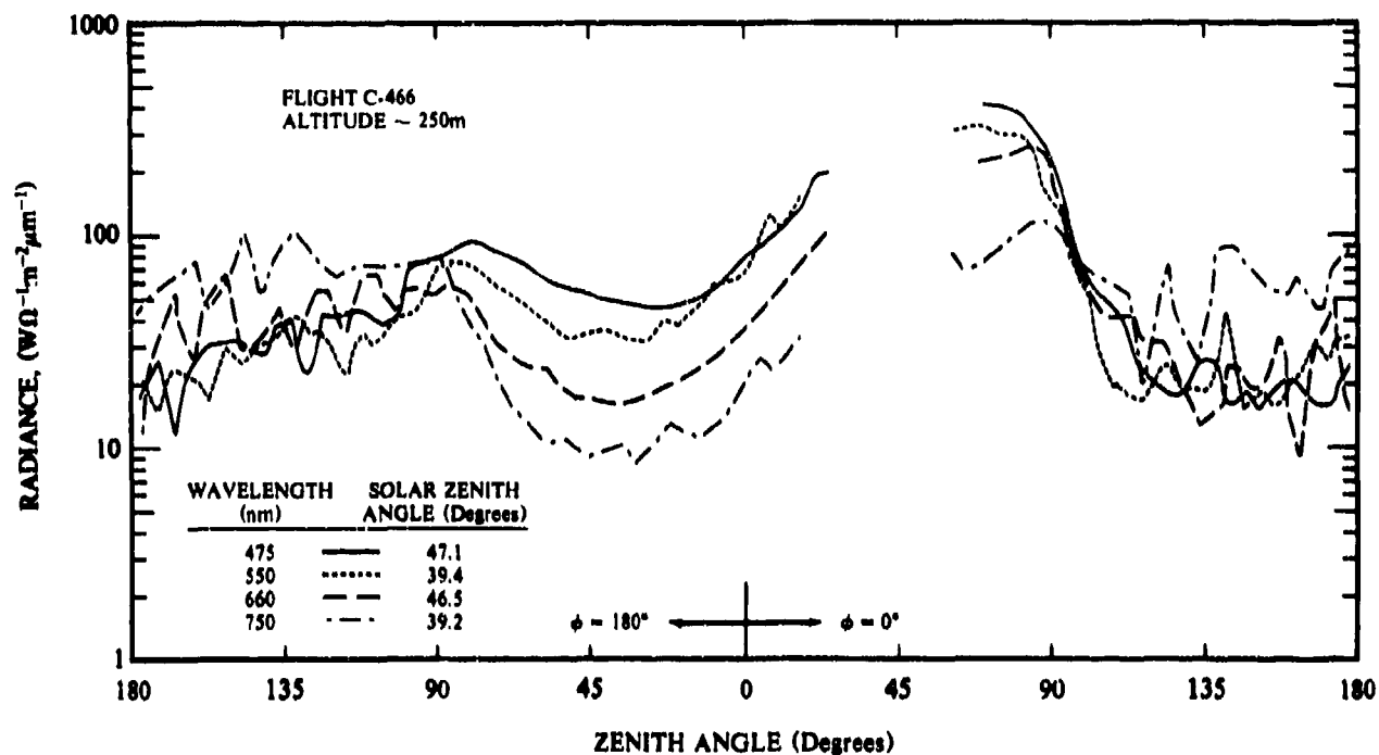
Fig. 4-9. Variation of Radiance Field with Wavelength, Flight C-466, z \approx 250\text{m AGL} , \phi = 0^\circ/180^\circ .
