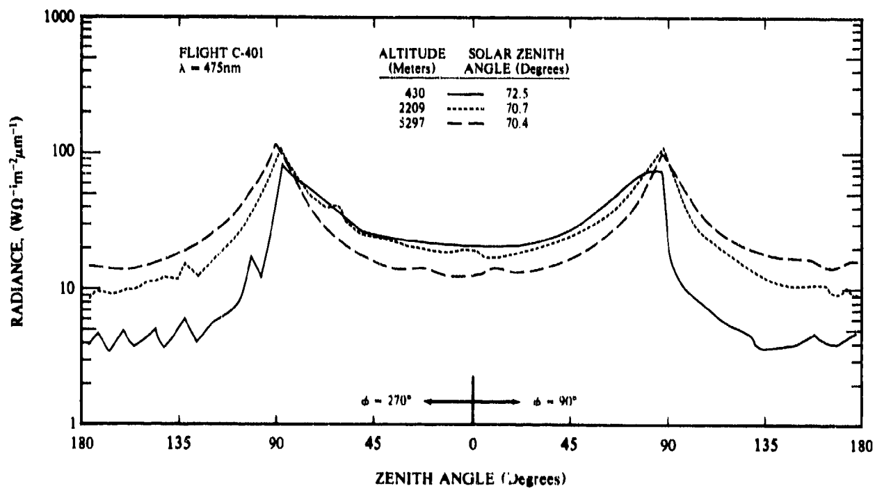
Fig. 4-6. Variation of Radiance Field with Altitude, Flight C-401, \lambda = 475\text{ nm} , \phi = 90^\circ/270^\circ .
