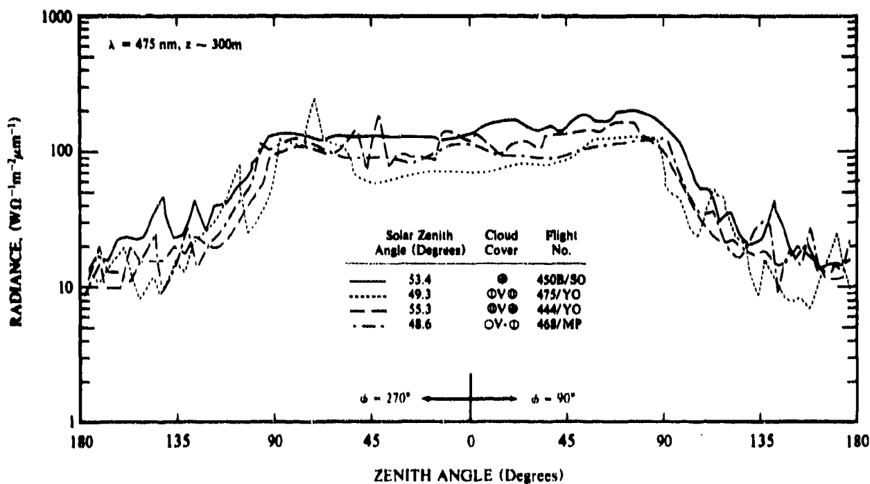
Fig. 4-18. Comparison of Radiance Measurements for Selected Flights with Variable Cloud Cover, \lambda = 475 \text{ nm} , z \approx 300\text{m} AGL, \odot\text{V}\odot , \phi = 90^\circ/270^\circ
