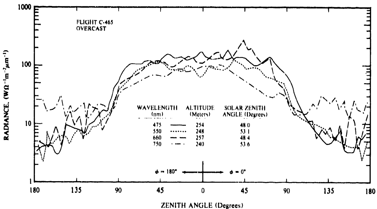
Fig. 4-24. Radiance Distribution as a Function of Wavelength for Overcast Sky Conditions, Flight C-465, z \approx 250 m AGL, \phi = 0^\circ/180^\circ .
