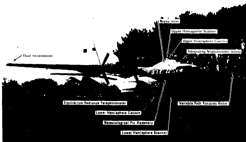
Fig. 2-1. C-130 Airborne Instrument System.
