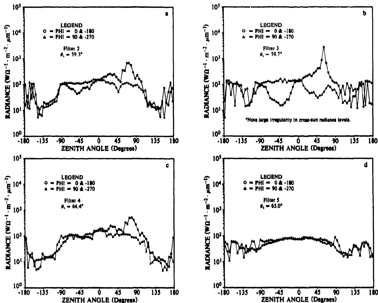
Fig. 3-6. Flight C-439 (Birkhof, Germany), Broken Cloud over Forest with Snow, 1600m AGL.
