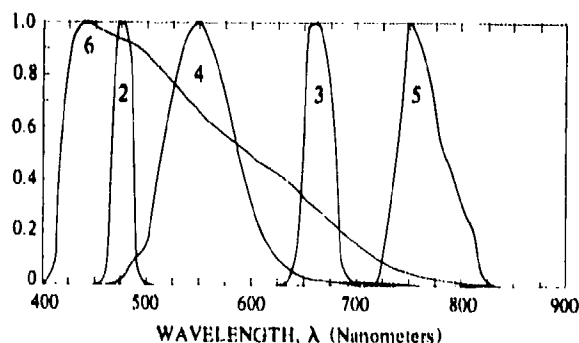
Fig. 2-3. Standard Spectral Responses. Peak Wavelengths are: 2 = 475nm Blue, 3 = 660nm Red, 4 = 550nm Photopic, 5 = 750nm N.I.R., 6 = 440nm S-20.
