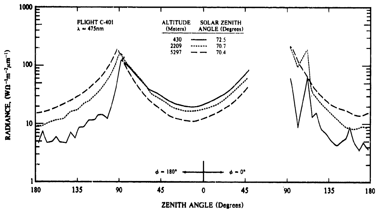
Fig. 4-5. Variation of Radiance Field with Altitude, Flight C-401, \lambda = 475\text{ nm} , \phi = 0^\circ/180^\circ .
