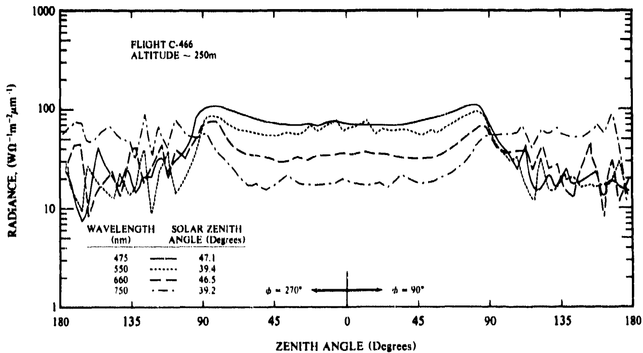
Fig. 4-10. Variation of Radiance Field with Wavelength, Flight C-466, z \approx 250\text{m AGL} , \phi = 90^\circ/270^\circ .
