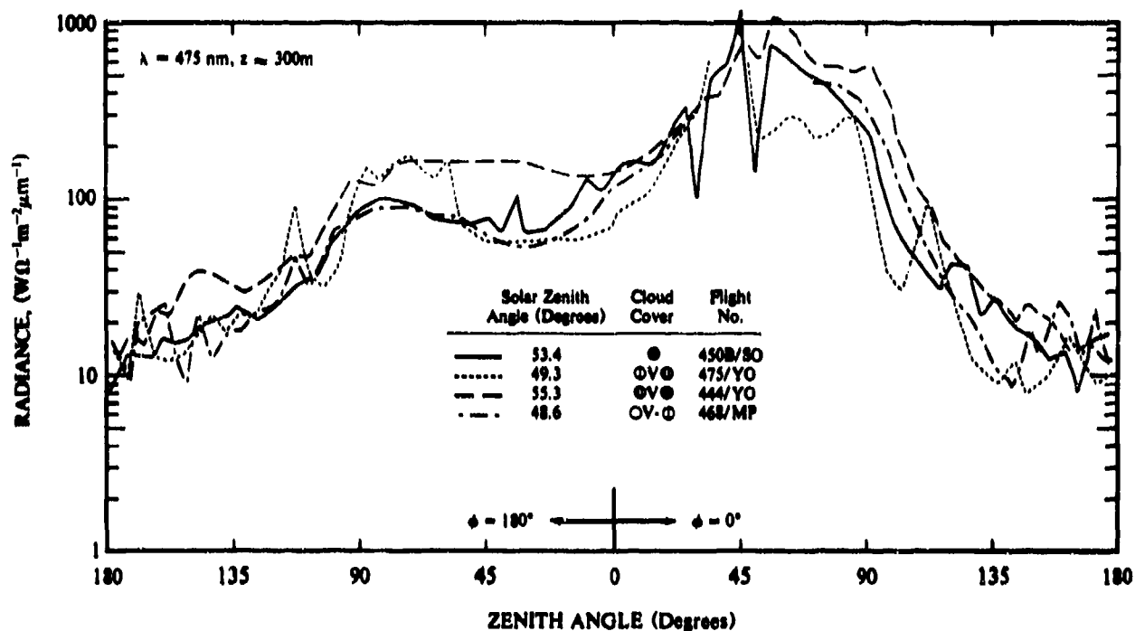
Fig. 4-17. Comparison of Radiance Measurements for Selected Flights with Variable Cloud Cover, \lambda = 475 \text{ nm} , z \approx 300\text{m} AGL, \odot\text{V}\odot , \phi = 0^\circ/180^\circ
