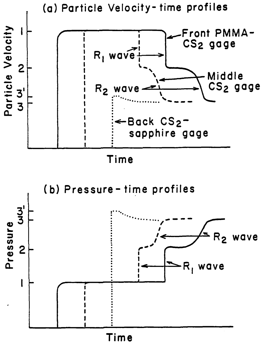
Fig. 1.5.--Wave Profiles Expected from a Three Gage Experiment. (a) shows particle velocity waveforms to be measured in the experiment. (b) shows corresponding pressure profiles although these are not measured or calculated in this study. The first and second reflected waves have labeled the R_1 wave and R_2 wave, respectively.
