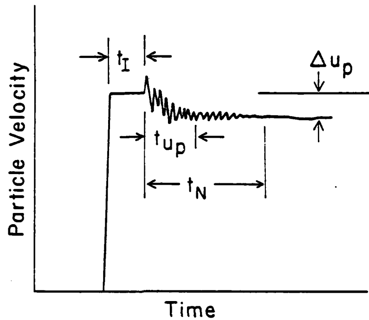
Fig. 4.5.--Idealized \text{CS}_2 -Sapphire Gage Record. t_I is the induction time, t_N is the noise decay time, t_{up} is the particle velocity decay time, and \Delta u_p is the particle velocity decrease.
