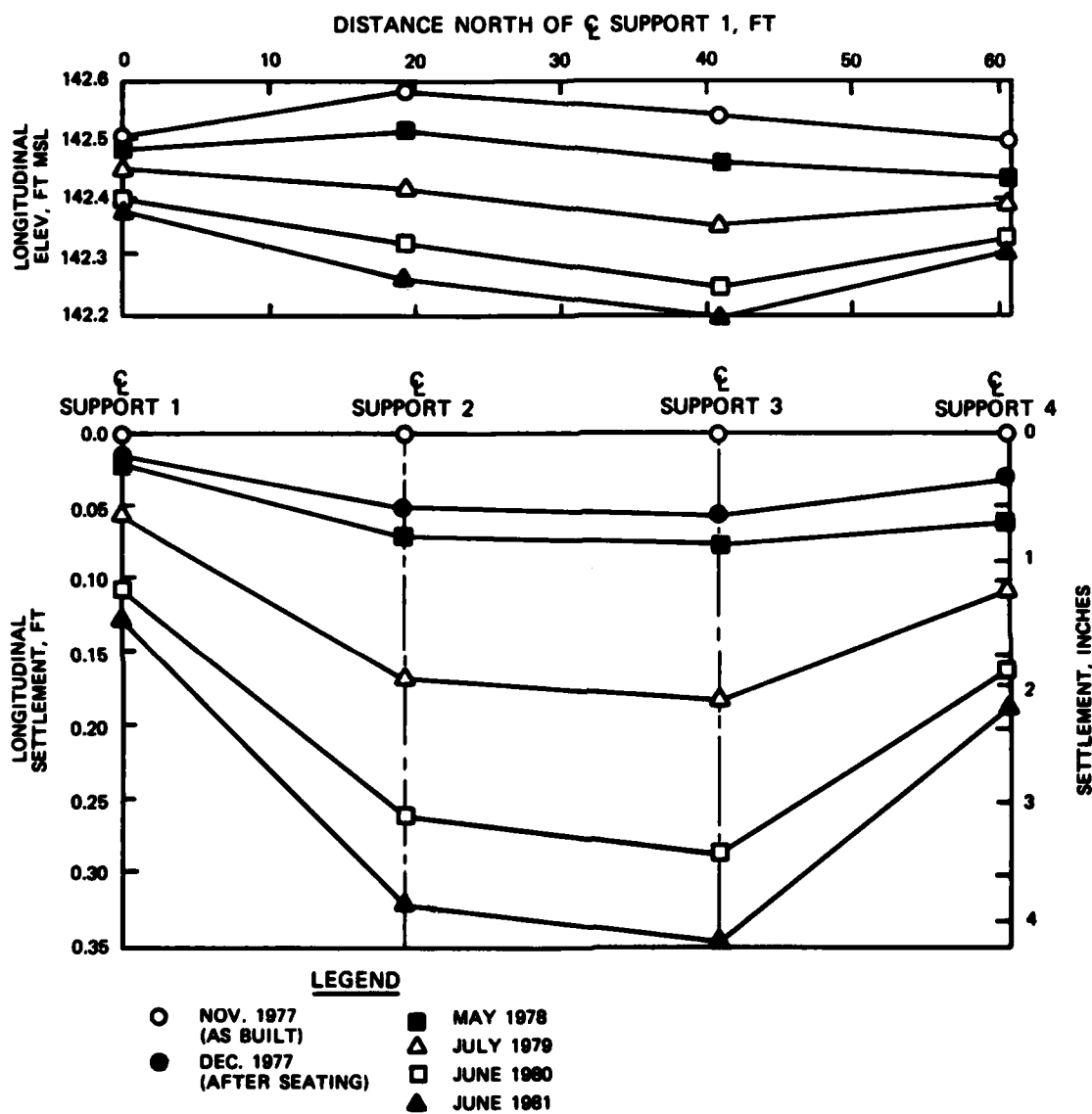
Figure 19. Summary of vertical bridge deck movement
