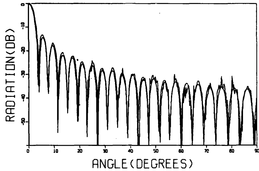
Fig. 1 — Comparison of antenna patterns with an exact solution and the one that uses a table of 32 entries
