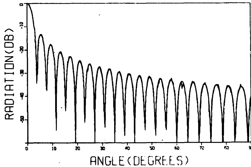
Fig. 2 — Comparison of antenna patterns with an exact solution and the one that uses a table of 128 entries
