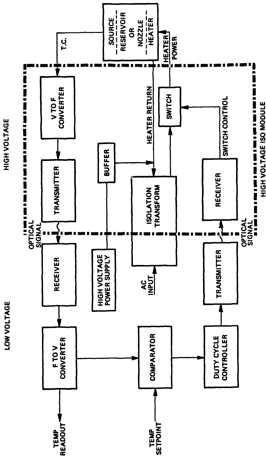
Fig. 2-20 Block Diagram of Thermocouple Isolation Circuitry
