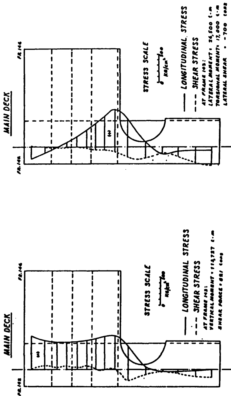
Figure 4-11 Stress Distribution Due to Wave-Induced Vertical Bending Fr. 142-146 Second Loading Case
