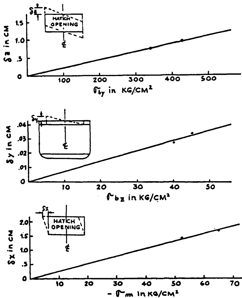
Figure 4-10 Hatch Distortion vs. Stresses in Transverse Box at Fr. 178, Port Side-Section B Due to Torsional and Lateral Moments For the SL-7 Containership
