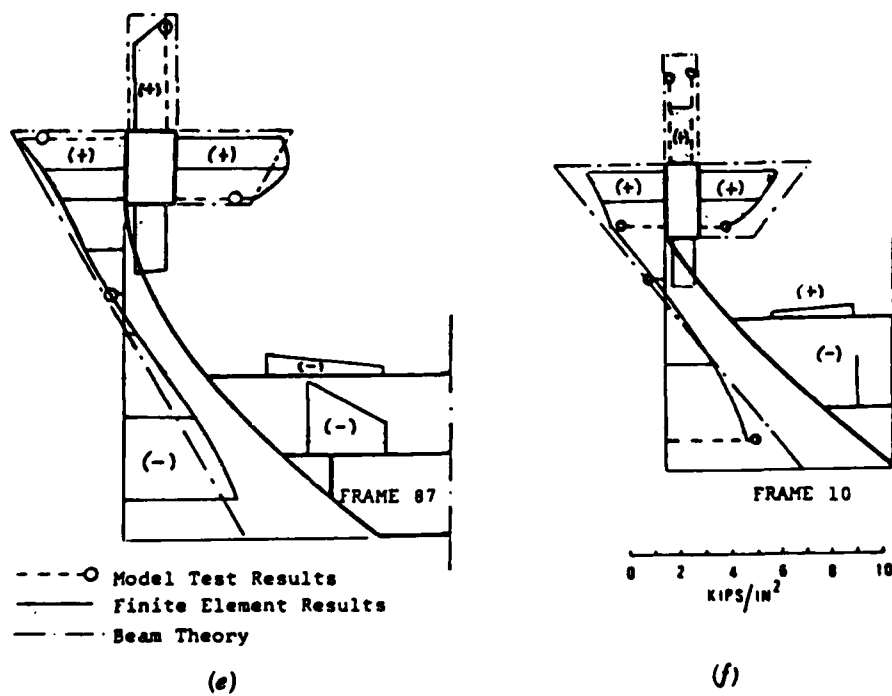
Figure 4-21 Comparisons of Structural Model Tests and Finite-Element Calculations for the SL-7 Containership, Loading Case 1.
