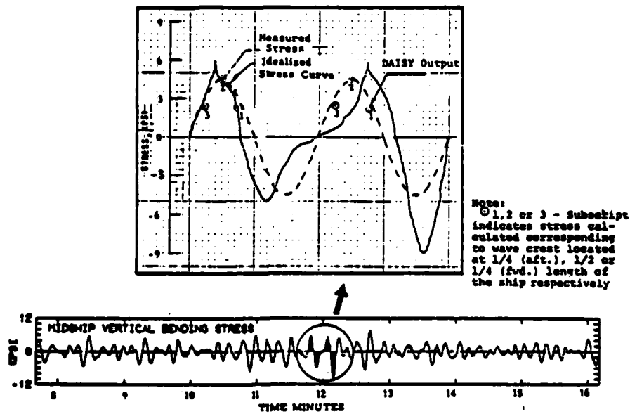
Figure 4-25 Comparison of the calculated and measured mean midship vertical bending stresses (Sensor LVB), Wave Condition 15
