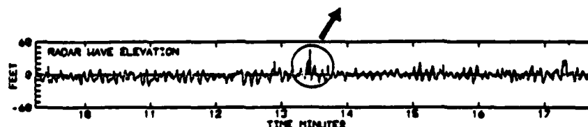
Figure 4-24 Comparisons of the wave time history measured on the SEA LAND McLEAN and the regular wave representations (Condition 16 - Voyage 32W - Tape 145 - Index 29 - Interval 50 - Run 450)
