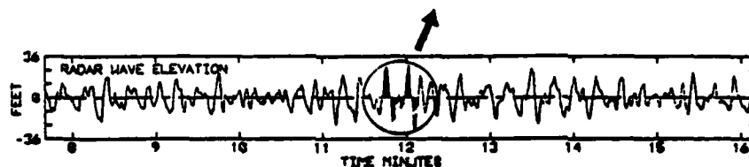
Figure 4-23 Comparisons of the wave time history measured on the SEA LAND McLEAN and the regular wave representations (Condition 15 - Voyage 32W - Tape 145 - Index 18 - Interval 5 - Run 405)
