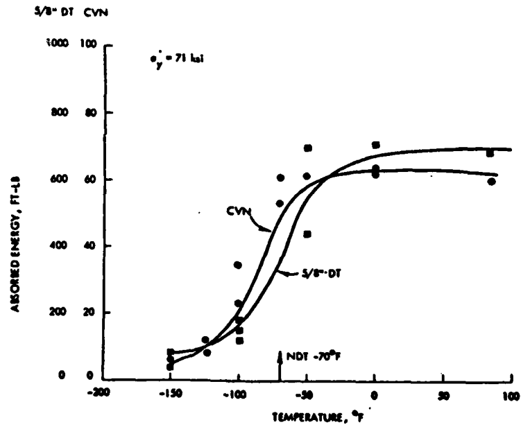
Figure 4.11 DT and CVN Test Results for A537B Steel \sigma_y = 71 \text{ ksi (490 MN/m}^2\text{)}
