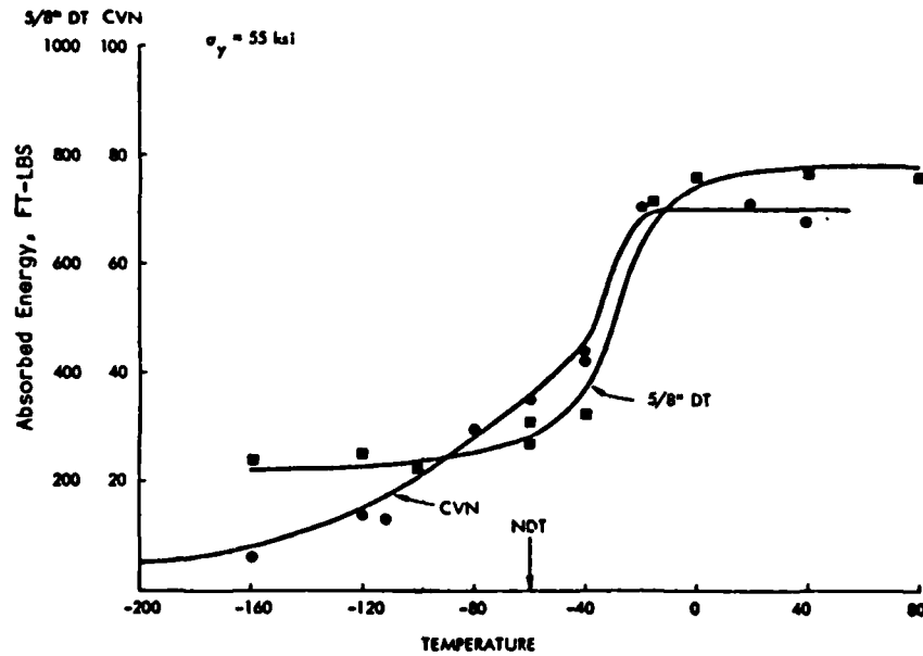
Figure 4.9 DT and CVN Test Results for 537A Steel -\sigma_y = 55 \text{ ksi} ( 379 \text{ MN/m}^2 )
