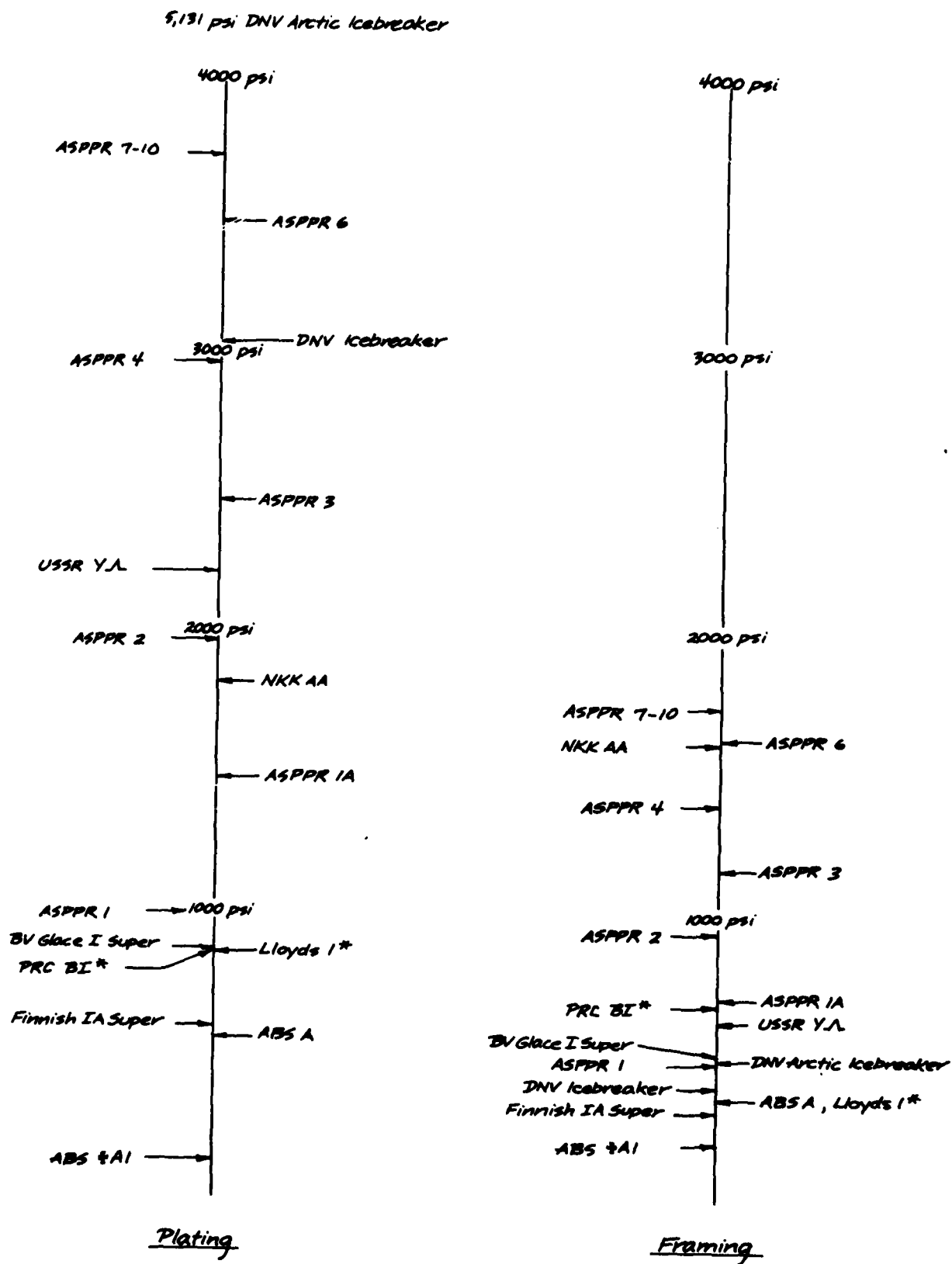
Figure 5.15 Load Carrying Capability of Arctic Tanker Bow Structure for Various Ice Strengthening Criteria
