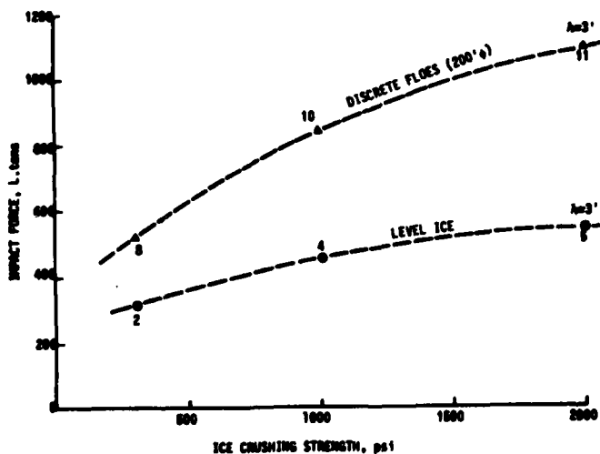
Figure 2.4 Effect of Crushing Strength in Crushing-Bending Failure Mode
