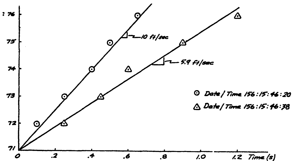
Figure 8.2 Polar Star Hull (Strain Gage) Response, 1976
