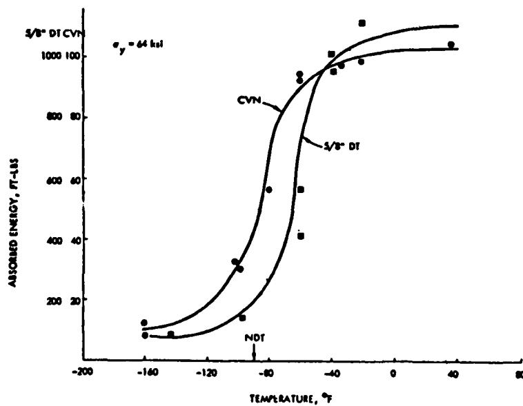
Figure 4.10 DT and CVN Test Results for A537B Steel -\sigma_y = 64 \text{ ksi} ( 441 \text{ MN/m}^2 )
