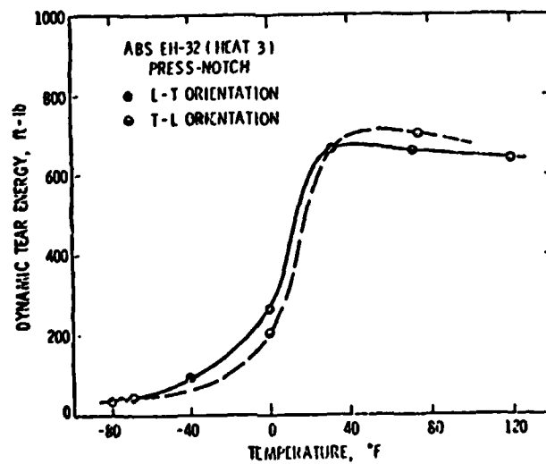
Figure 4.8 EH-32 (Heat3), 5/8" Parent DT, Press-Notch
