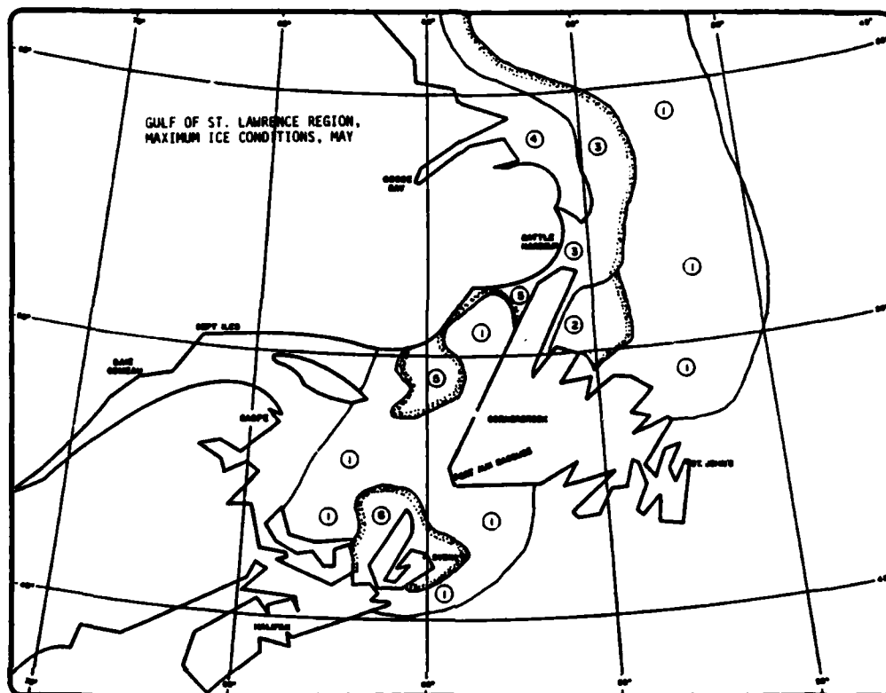
MAXIMUM ICE CONDITIONS, MAY
