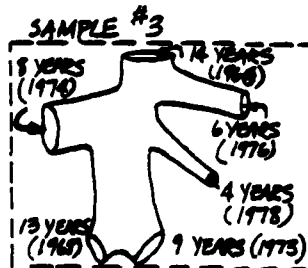
Fig. 11. Buttress root ages and relationships with sediments.
