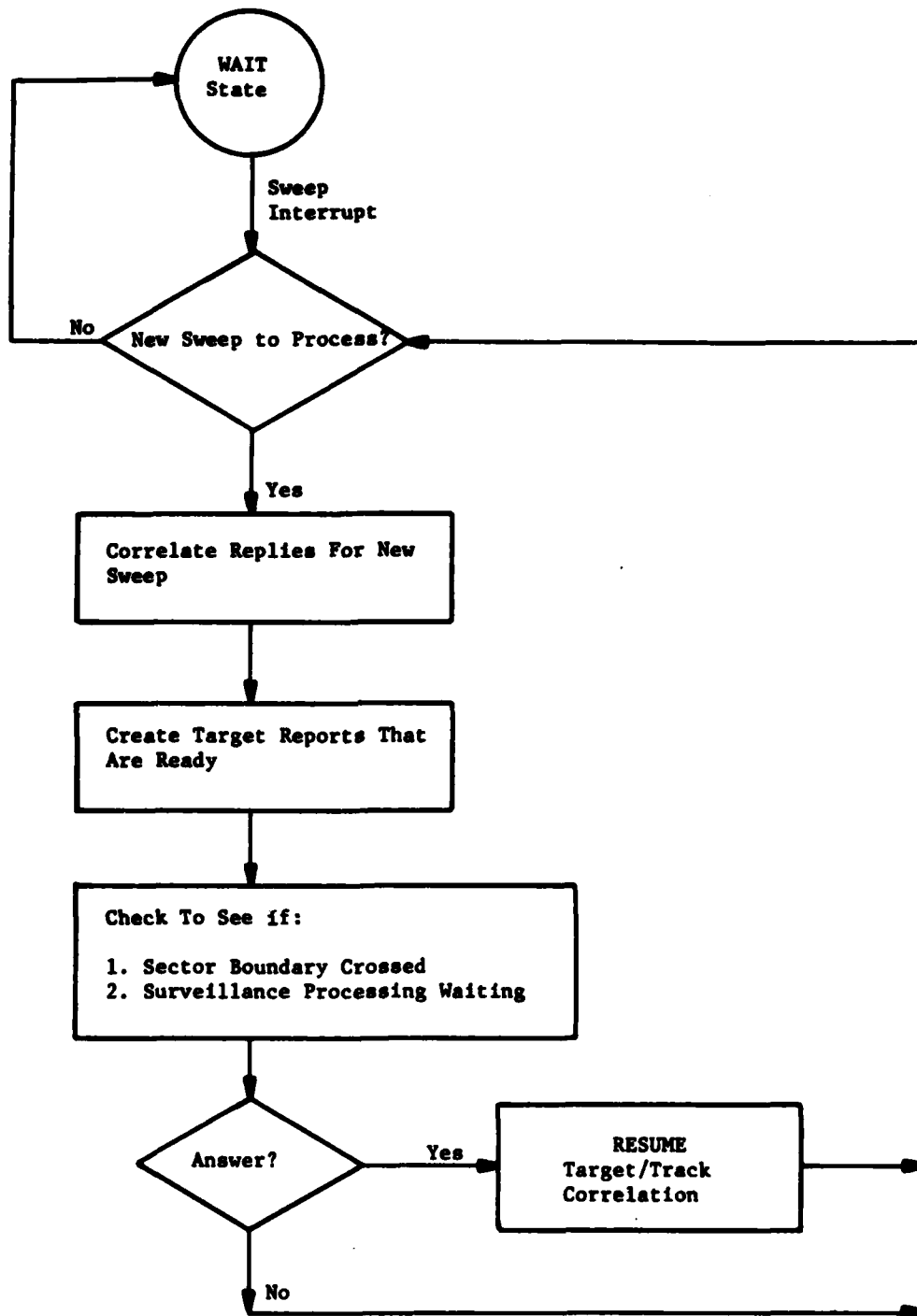
Fig. 5-2. Reply Correlation Task.
