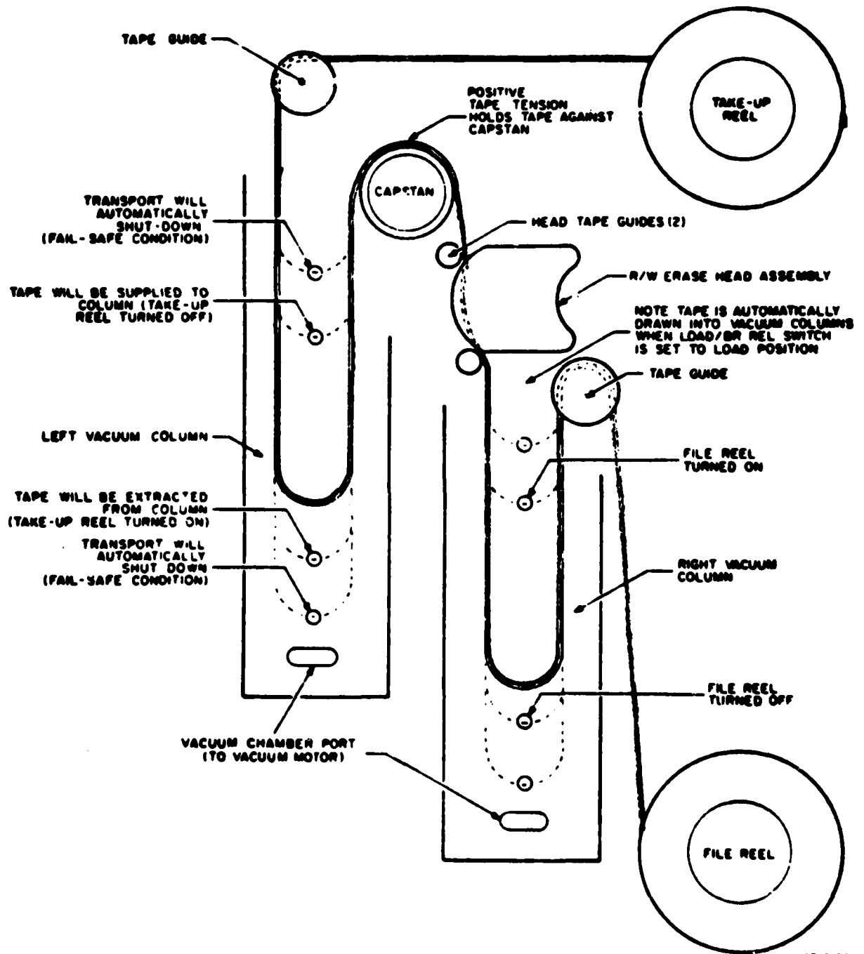
Fig. 10-5. Tape Threading.
