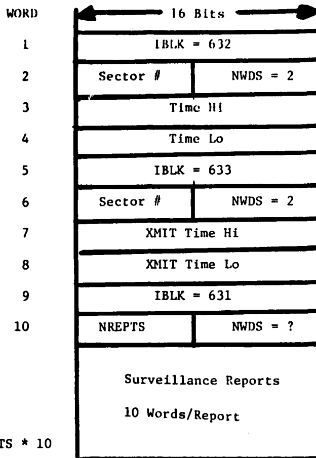
Fig. 8-1. Surveillance Output Buffer.
