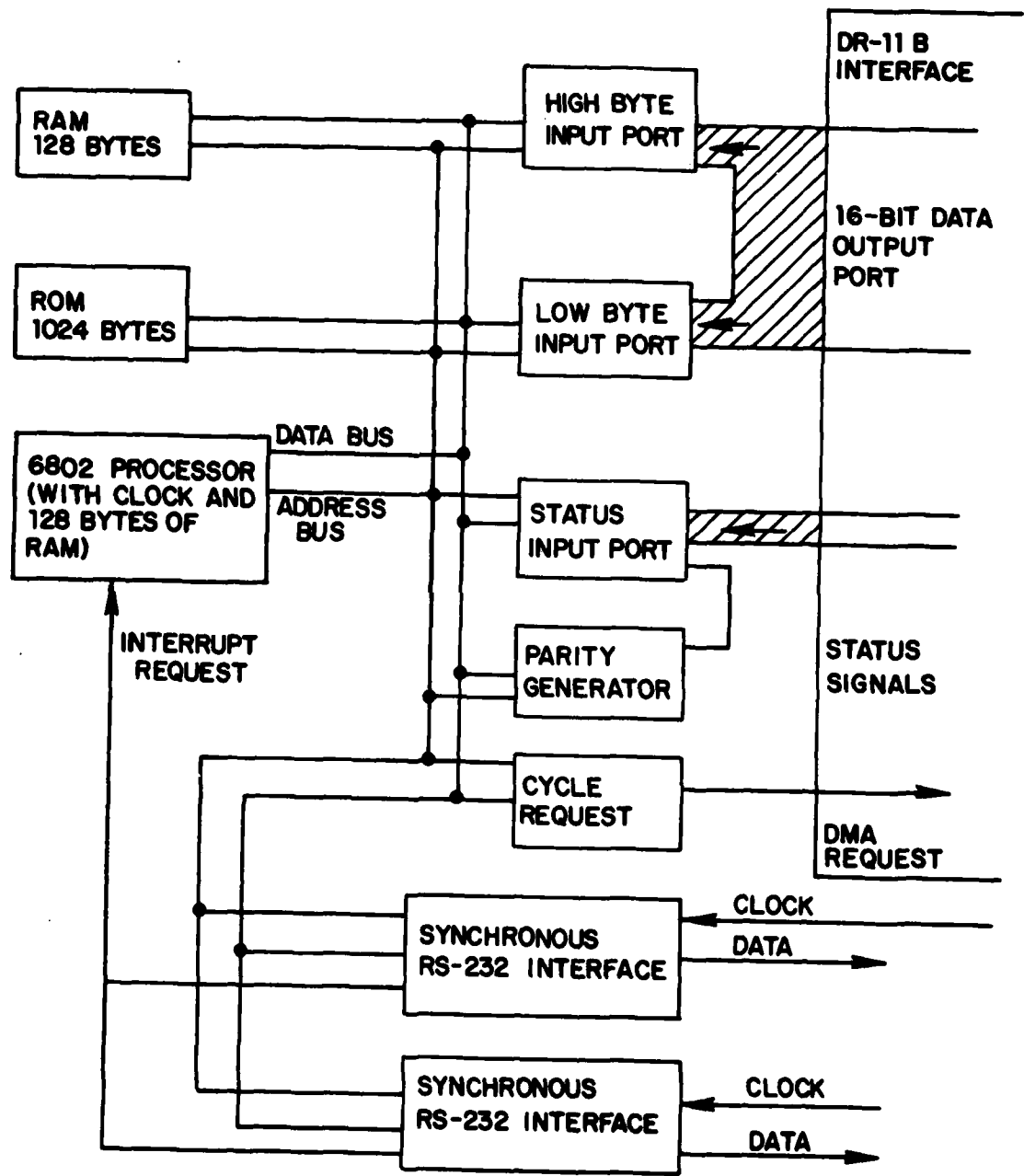
Fig. 9-1. Microprocessor Interface.
