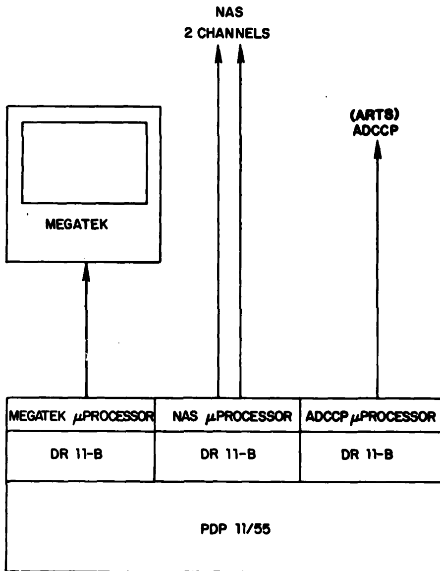
Fig. 9-2. Interface Data Lines.
