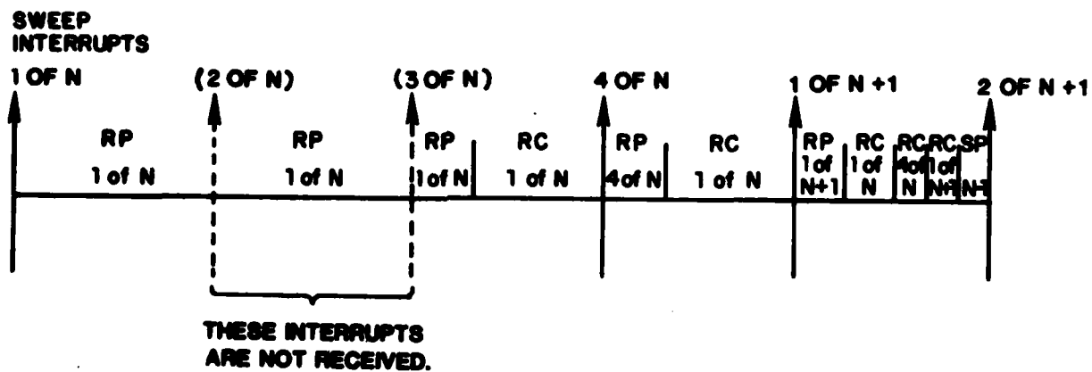
Fig. 5-7. Reply Processing Falls Behind.
