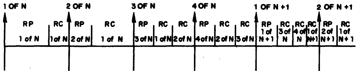
Fig. 5-8. Reply Correlation Falls Behind.
