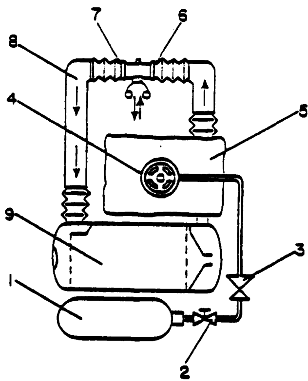
Figure 1. Functional Schematic
