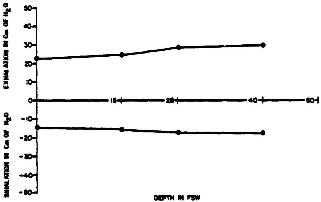
Figure 18. OKYMAX 3, OPEN-CIRCUIT DEMAND MODE PEAK DIFFERENTIAL PRESSURES vs. DEPTH AT 62.5 RMV
