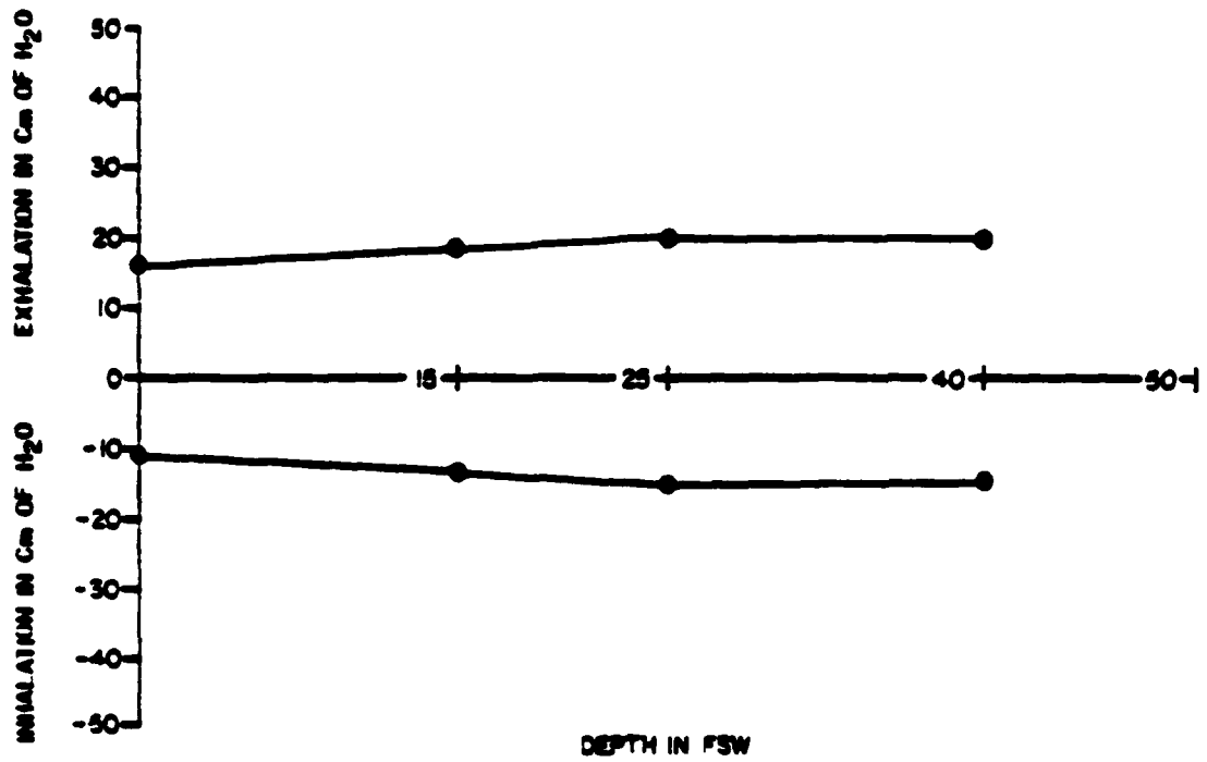
Figure 17. OKYMAX 3, OPEN-CIRCUIT DEMAND MODE PEAK DIFFERENTIAL PRESSURES vs. DEPTH AT 40.0 RMV
