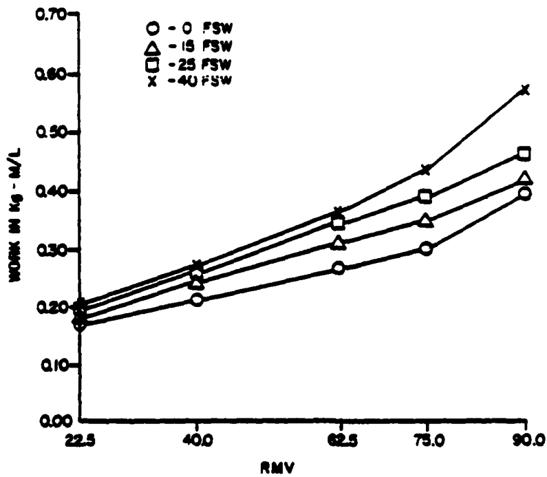
Figure 35. OXYMAX 3, OPEN-CIRCUIT MODE BREATHING WORK vs. RMV
