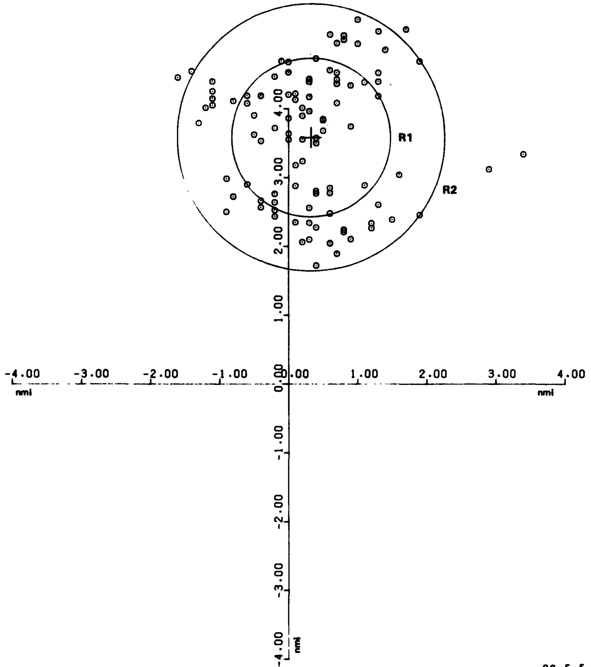
FIGURE 5. EN ROUTE FLIGHT, TRELAW, ARGENTINA TO RIO DE JANEIRO, SCATTER PLOT OMEGA SET 01 VERSUS INS
