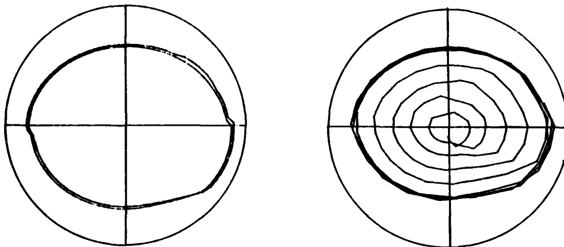
Figure 2-5: Total energy plotted in polar form. Radius is magnitude of energy, angle is \text{Arctan}(\dot{y}_2/\dot{y}_1) . Left) Data of Figure 2-4 replotted. Right) Period during which hopping height increases. (Circles indicate 50 joules.)
