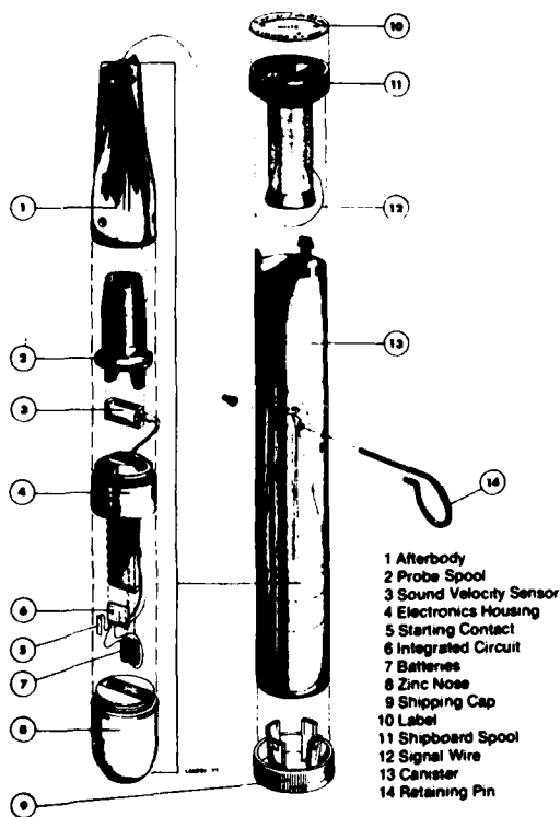
XSV Exploded View
