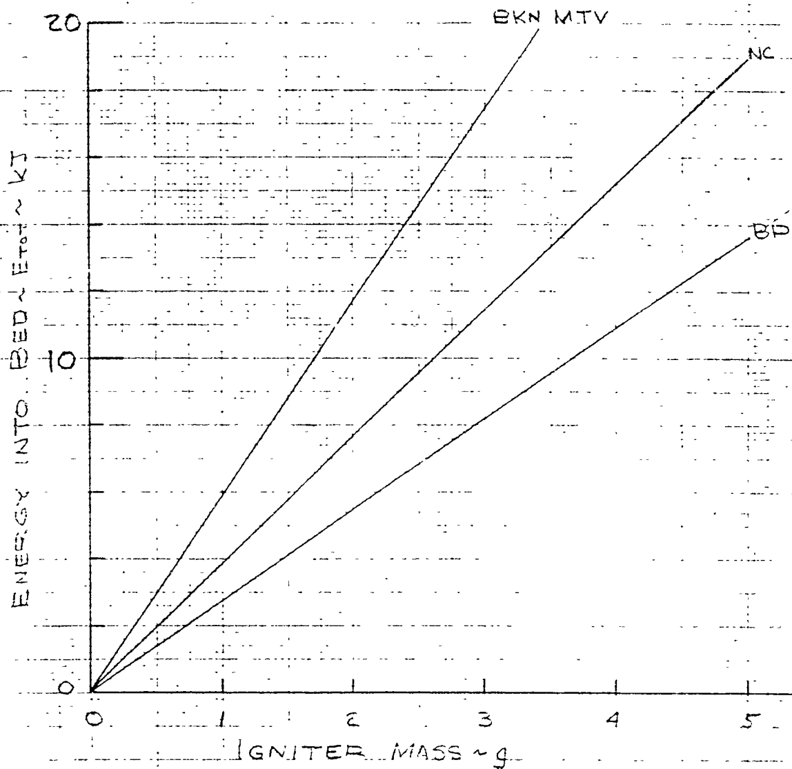
Figure D-12 Calculated Igniter Performance Characteristics: Total Energy into Bed
