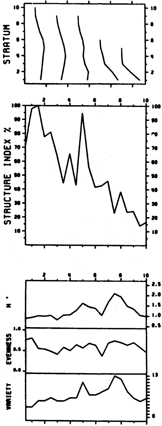
Figure B14. (Concluded)
