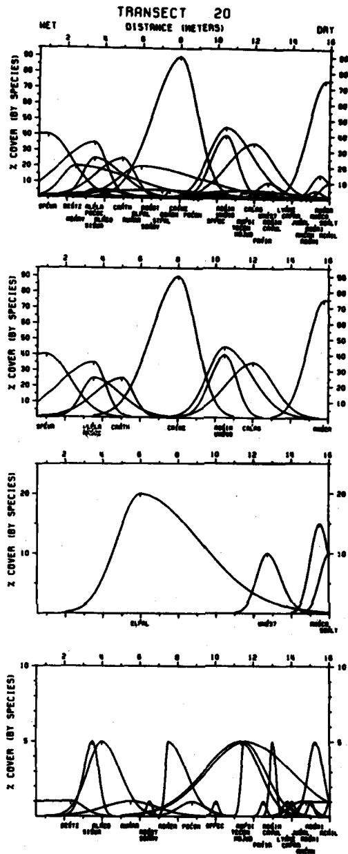
Figure 14. Cover by species along transect 20 at pond 3 at Ordway Prairie. The top graph includes all species occurring along the transect, the second graph includes species with maximum cover values >30 percent, the third >5 percent, and the fourth <5 percent. Tick marks at the peak of each curve correspond directly below to a species mnemonic code. Where tick marks on curves are superimposed vertically, the mnemonic code nearest the x-axis corresponds to the curve of maximum height, and so on. See Appendix C for translation of mnemonic codes for species
