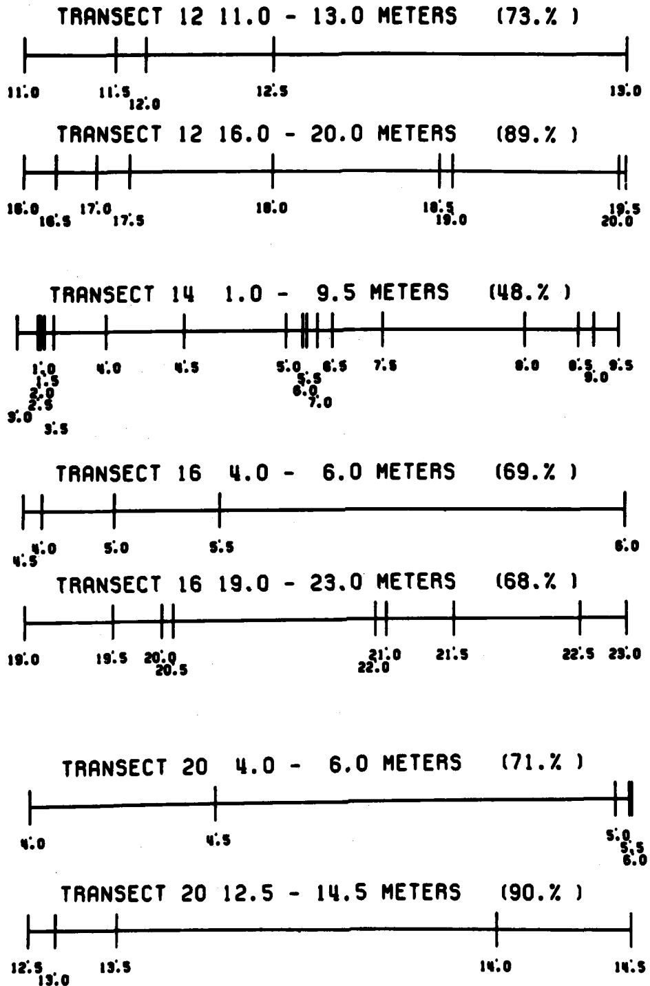
Figure 9. Ordination models (x-axis only) for upper and lower transitions of transects 12, 14, 16, and 20 following the technique of Swan, Dix, and Wehrhahn (1969)
