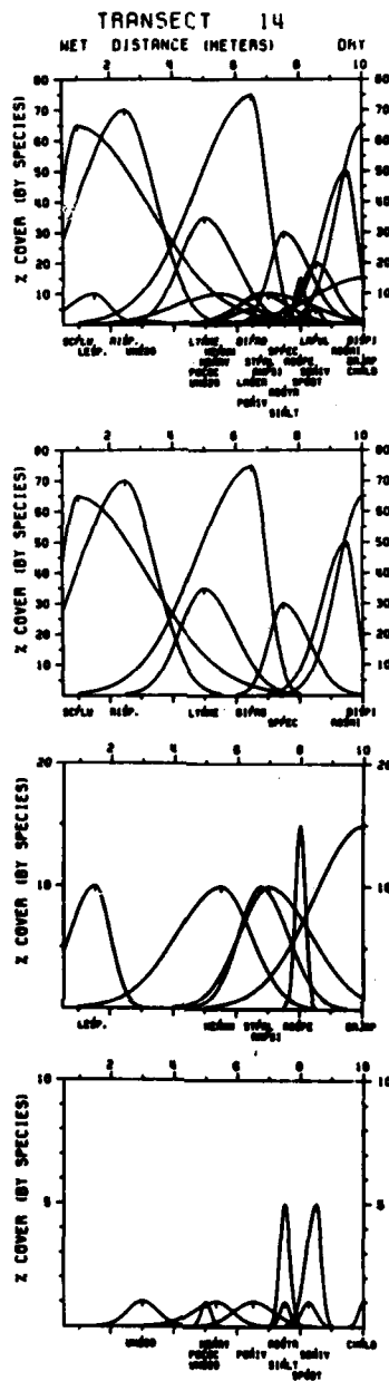
Figure 11. Cover by species along transect 14 at Platte Lake. The top graph includes all species occurring along the transect, the second graph includes species with maximum cover values >30 percent, the third >5 percent, and the fourth <5 percent. Tick marks at the peak of each curve correspond directly below to a species mnemonic code. Where tick marks on curves are superimposed vertically, the mnemonic code nearest the x-axis corresponds to the curve of maximum height, and so on. See Appendix C for translation of mnemonic codes for species
