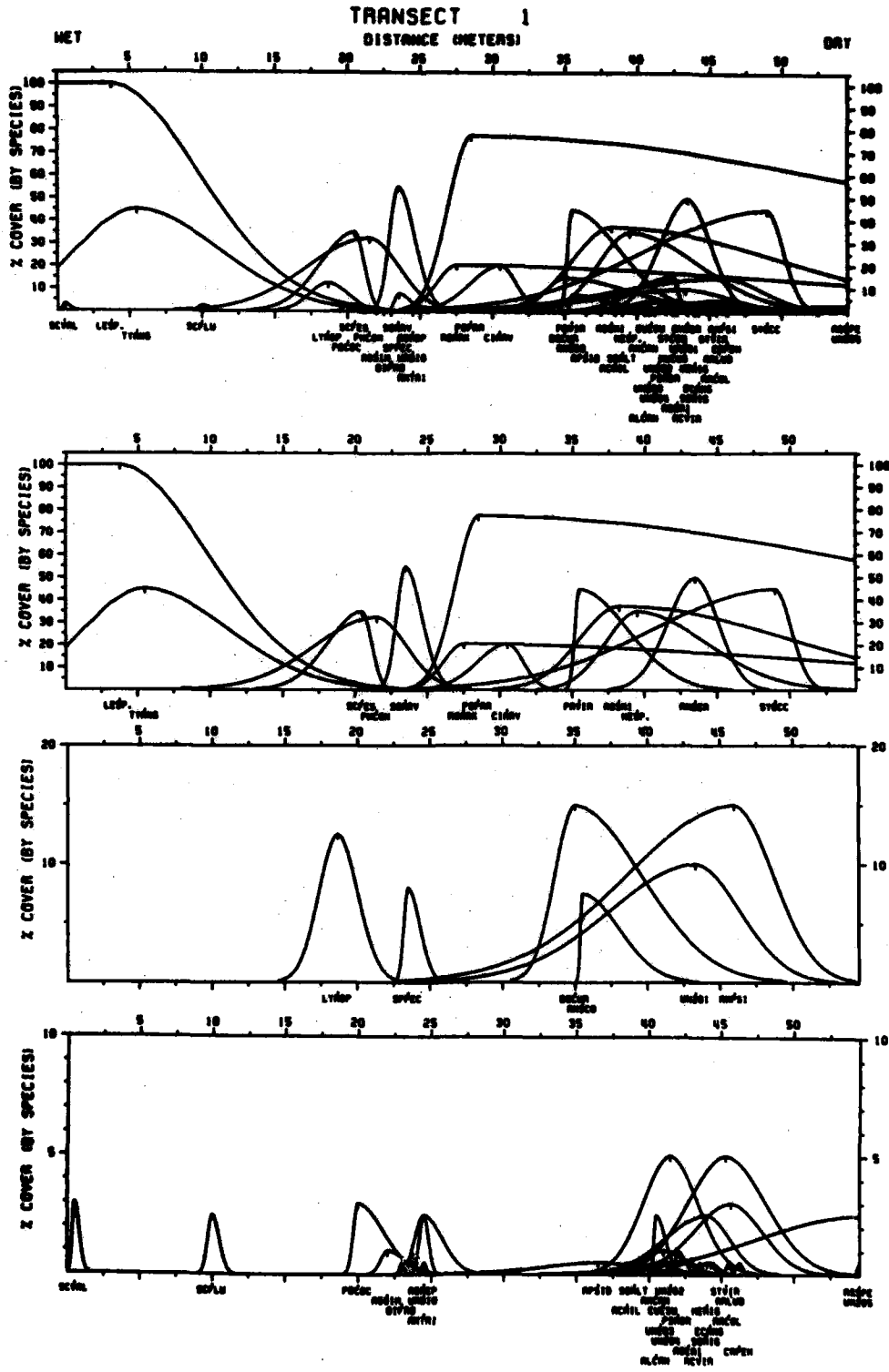
Figure B1. Direct gradient analysis graph, transect 01 (Continued)
