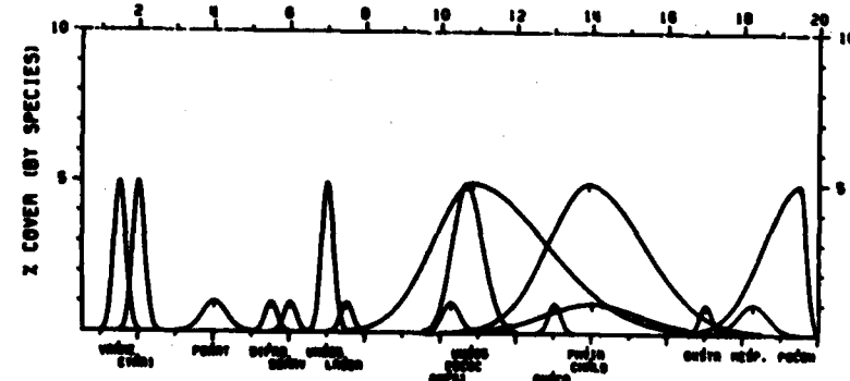
Figure B10. Direct gradient analysis graph, transect 10 (Continued)
