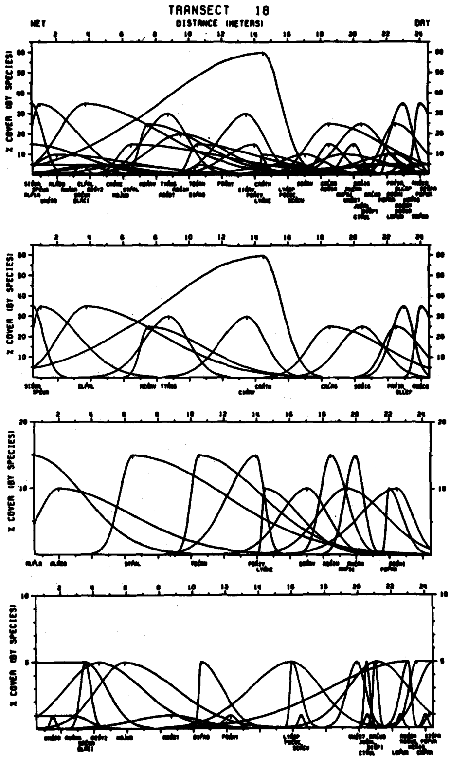
Figure B18. Direct gradient analysis graph, transect 18 (Continued)
