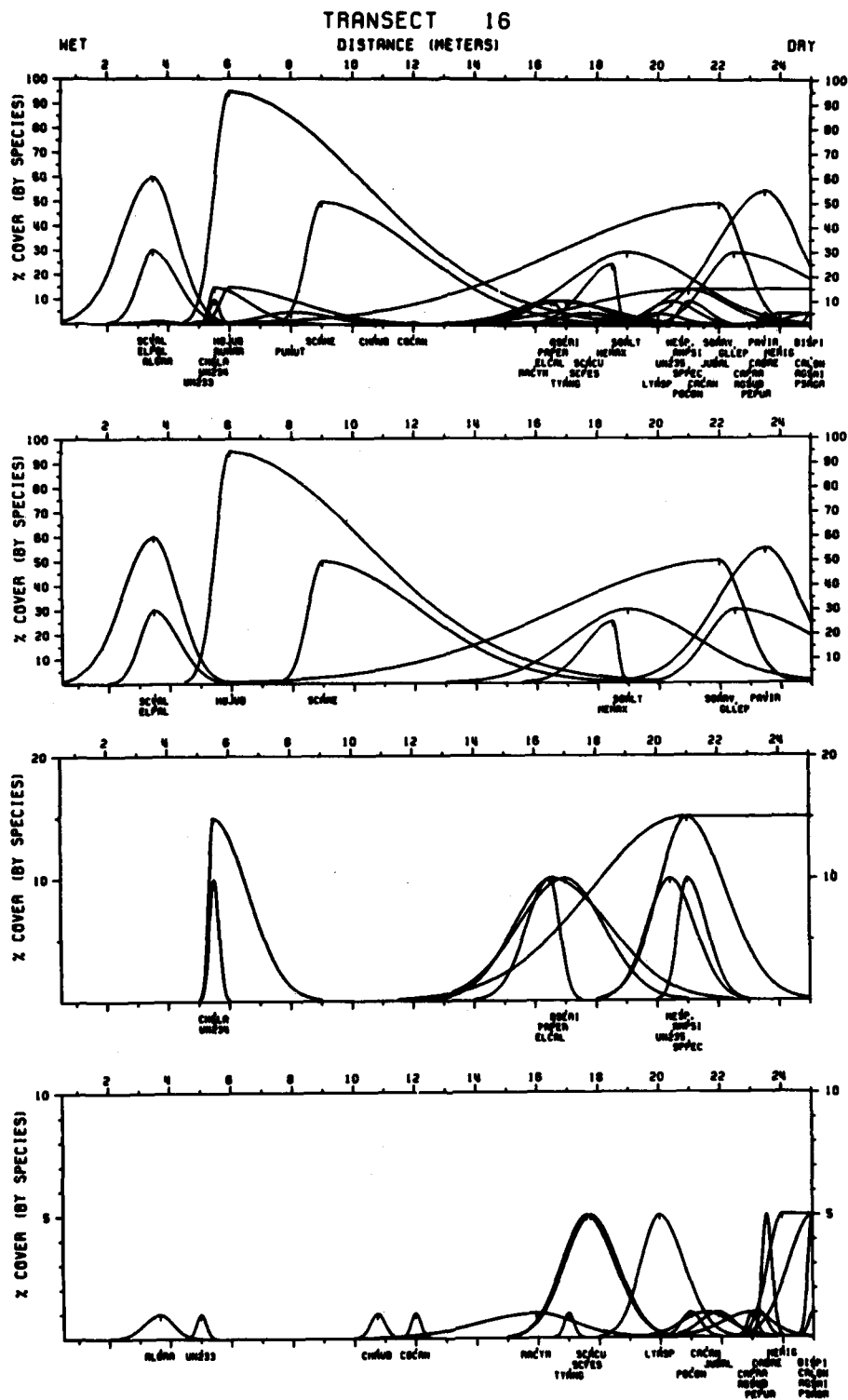
Figure B16. Direct gradient analysis graph, transect 16 (Continued)
