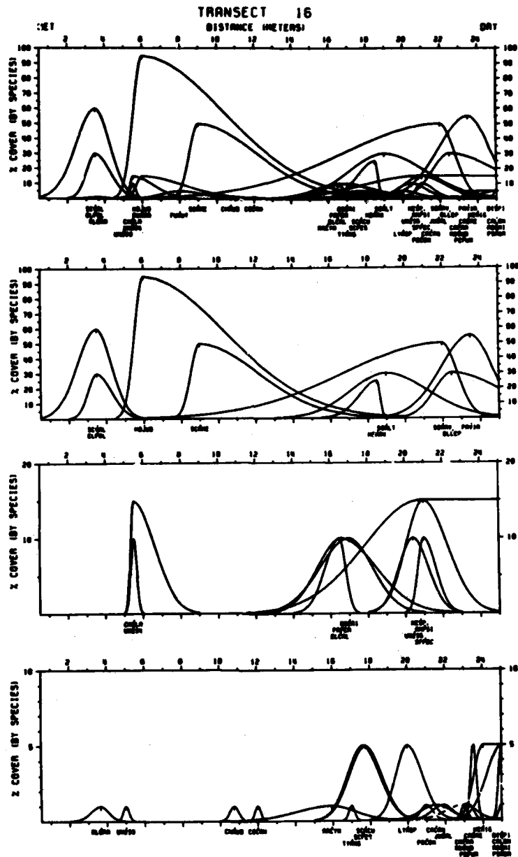
Figure 12. Cover by species along transect 16 at pond 1 at Ordway Prairie. The top graph includes all species occurring along the transect, the second graph includes species with maximum cover values >30 percent, the third >5 percent, and the fourth <5 percent. Tick marks at the peak of each curve correspond directly below to a species mnemonic code. Where tick marks on curves are superimposed vertically, the mnemonic code nearest the x-axis corresponds to the curve of maximum height, and so on. See Appendix C for translation of mnemonic codes for species
