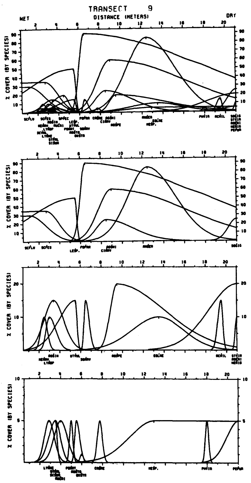
Figure B9. Direct gradient analysis graph, transect 09 (Continued)
