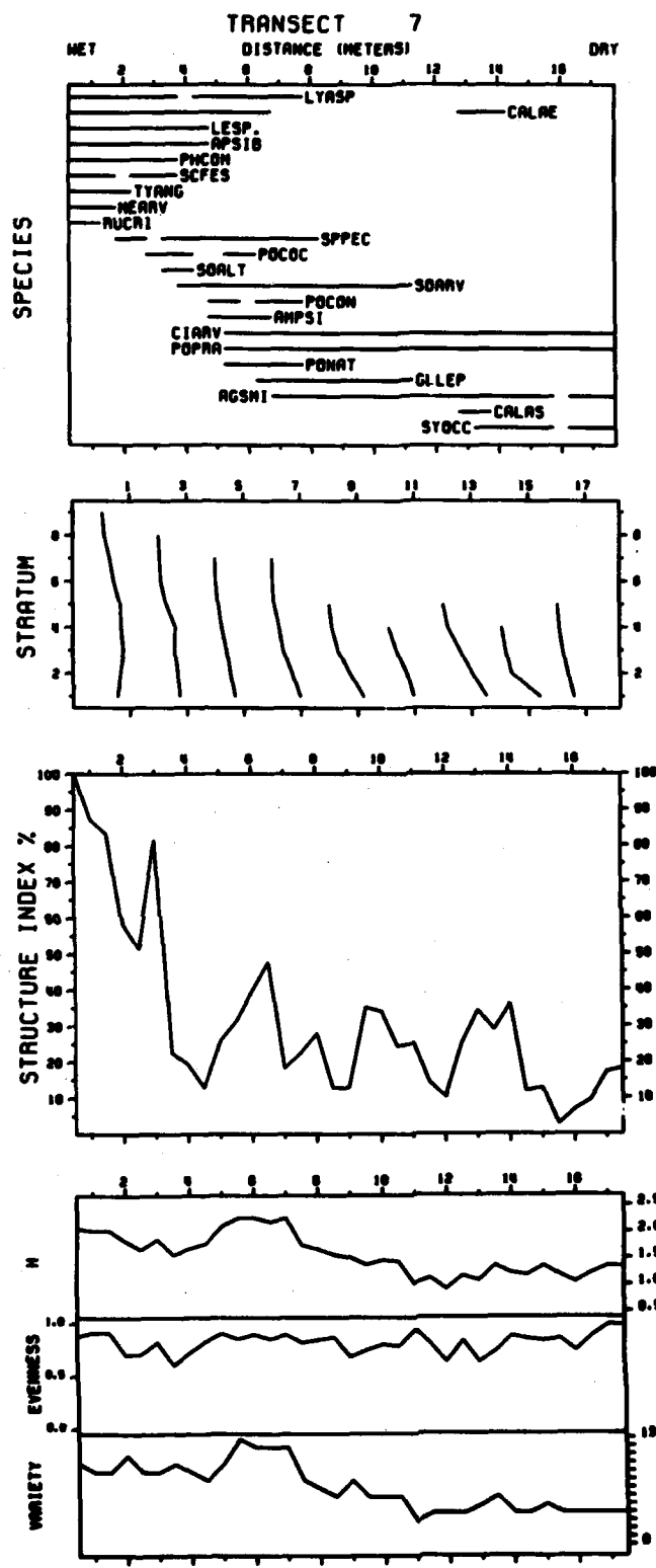
Figure B7. (Concluded)
