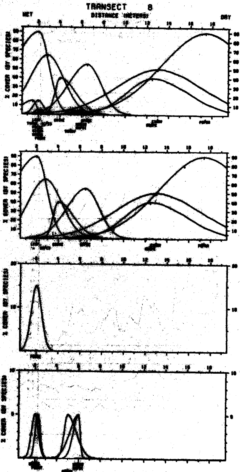
Figure B9. Direct gradient analysis graph, transect 08 (Continued)
