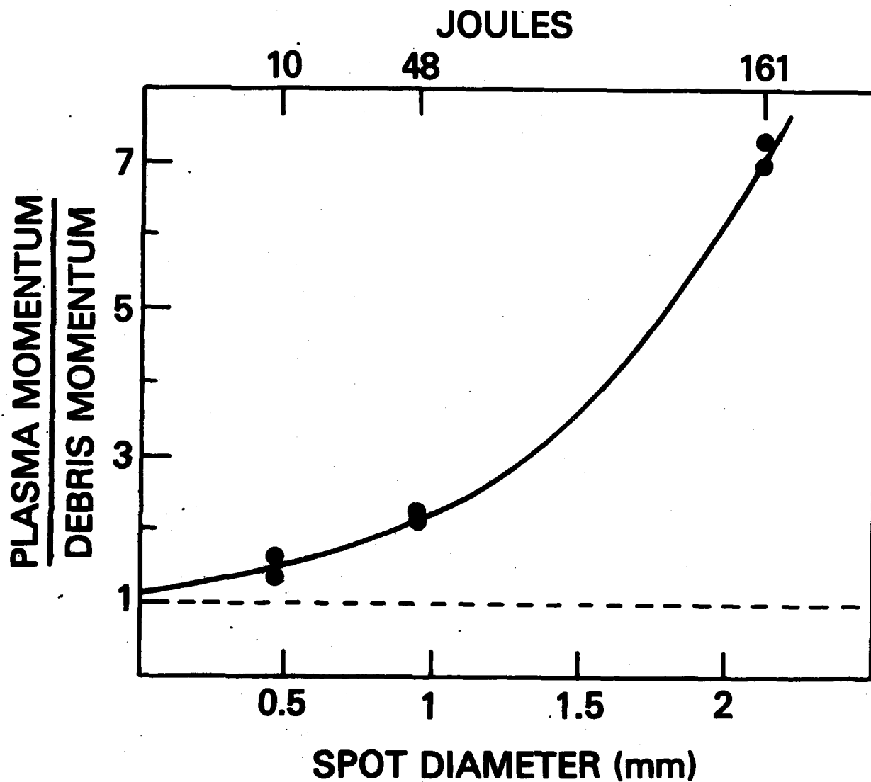
Fig. 5 — Ratio of plasma momentum to target debris momentum as a function of laser-spot diameter. The target is a 30 \mu\text{m} thick CH foil irradiated at 1 \times 10^{12} \text{ W/cm}^2 .
