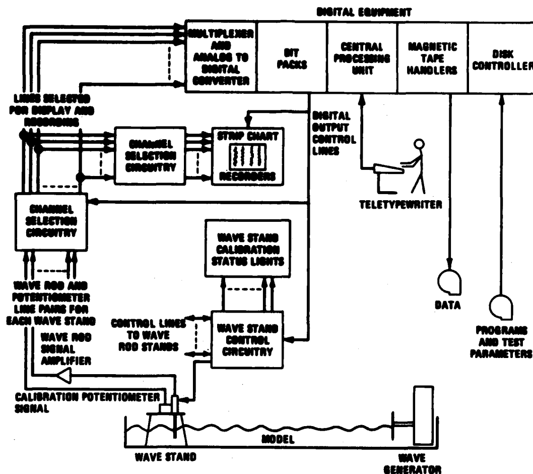
Figure 7. Automated Data Acquisition and Control System (ADACS) water-surface elevation with respect to time. The magnetic tape output was then analyzed to obtain the required data.
