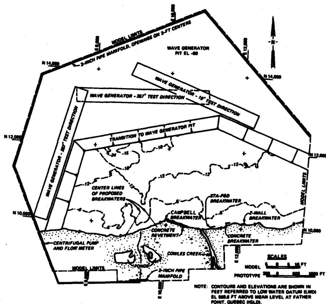
Figure 5. Model layout
