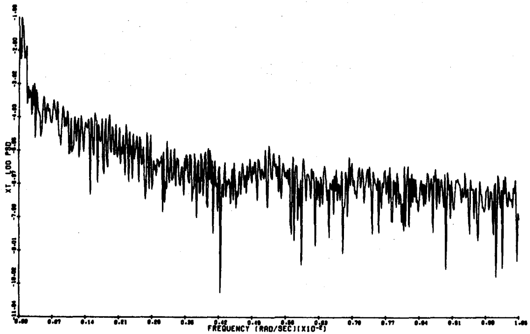
Figure 18. Spectral Analysis, X Translation
