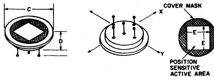
Figure 6. Photodiode
