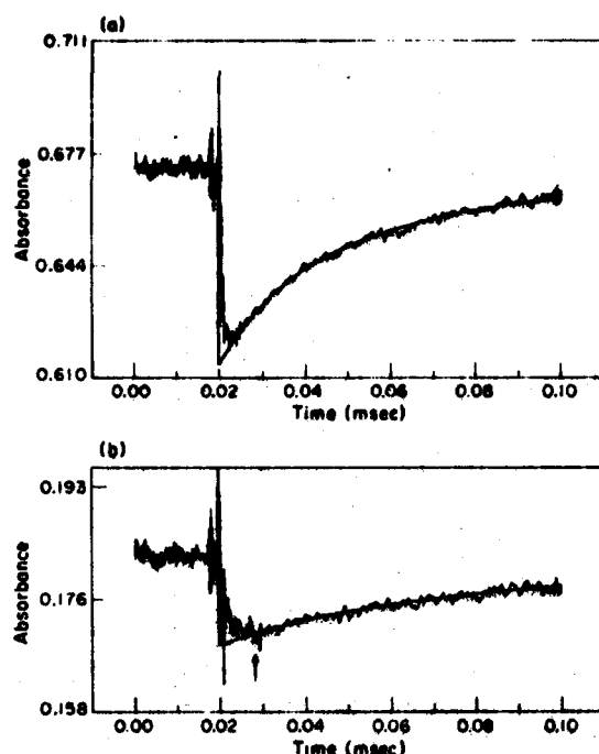
Fig. 2. Typical laser-induced absorbance transients in ozone at 254 nm. (a) Experimental and calculated transients at [O_2] = 29.5 Torr, [O_3] = 0.34 Torr, showing double exponential decay. (b) Experimental and calculated transients at [O_2] = 12.9 Torr, [O_3] = 0.16 Torr, showing "induction time" t_{ind} denoted by arrow. In both cases the decaying portion was digitally smoothed.
