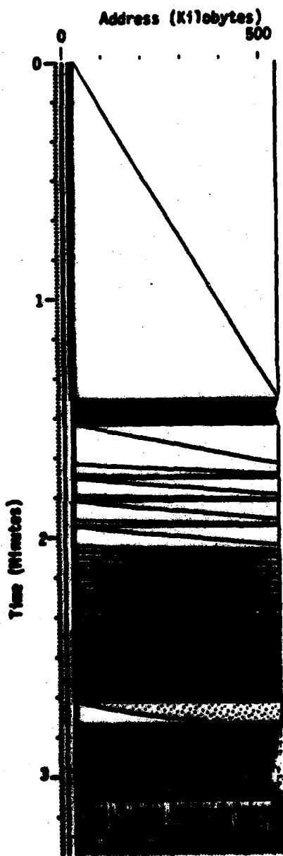
Figure 2: FFT Part 1
