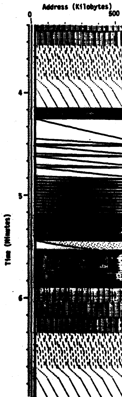
Figure 3: FFT Part 2
