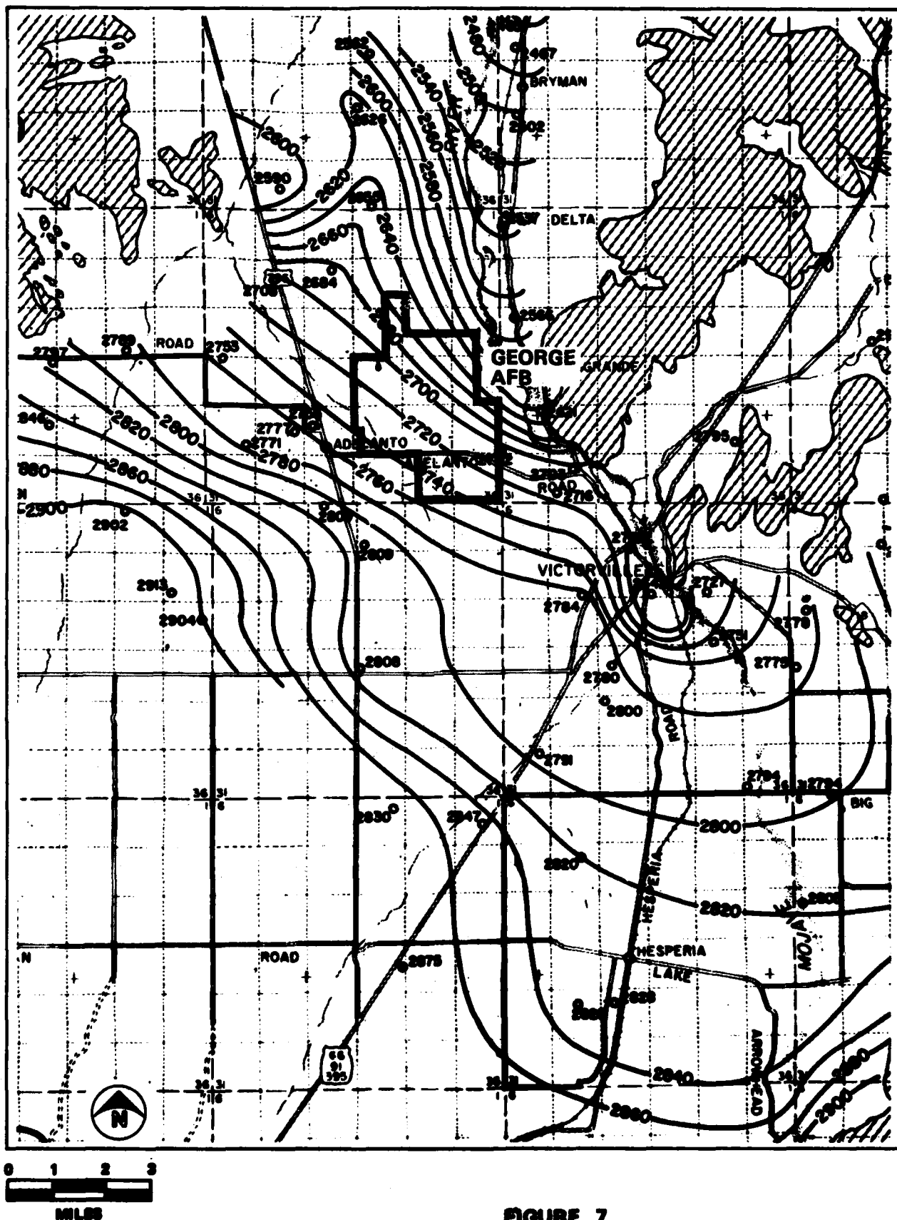
FIGURE 7 POTENTIOMETRIC SURFACE, 1964, GEORGE AFB AND VICINITY (California Dept. of Water Resources, Bulletin 84, 1967)
