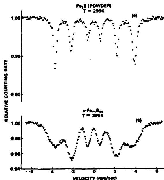
Fig. 1. (a) Spectrum of \text{Fe}_2\text{B} polycrystalline powder compared with (b) spectrum of \alpha\text{-Fe}_{71}\text{B}_{29} sputtered film, both at room temperature.
