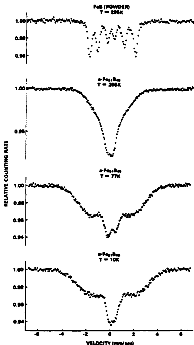
Fig. 2. Spectra of a\text{-Fe}_{81}\text{B}_{19} sputtered film at various temperatures compared with FeB polycrystalline powder at room temperature.
