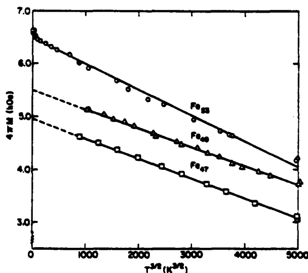
Fig. 1. Temperature dependence of the magnetization deduced from FMR data on amorphous Fe x B 1-x alloys. As described in the text, below 80 K, Fe 47 and Fe 49 do not show simple behavior. Hence, the dashed lines.
