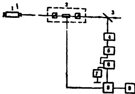
Figure 1. Principle of power stabilizer 1--He-Ne laser; 2--lithium niobate electric light switch; 3--beam splitter; 4--photo-electric tube; 5--current voltage converter; 6--comparative amplifier; 7--base voltage; 8--differential circuit; 9--high voltage
