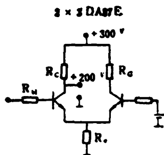
Figure 5. Differential circuit
