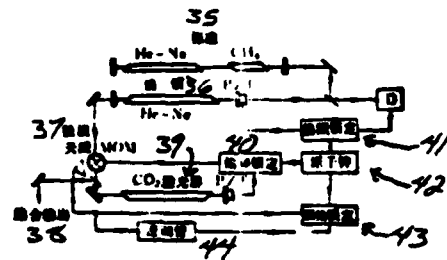
Figure 6. Optical frequency combination 35--standard; 36--lock; 37--microwave antenna; 38--combined output; 39--CO 2 laser; 40--frequency lock-in; 41--atomic clock; 42--frequency lock-in; 43--frequency lock-in; 44--velocity adjustment tube
