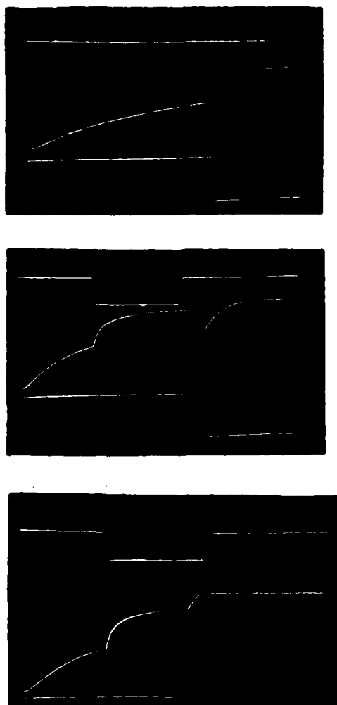
Fig. 1. Dynamic of structure's performance: a) no light pulse, b) recording of information, c) erasure of information. Lower beam is the electric-field pulse ( U=200 V), upper beam - pulse of an He-Cd laser lasting 10 ms ( I \sim 4 mW/cm 2 ), and middle beam - electrical-response signal (relative units).
