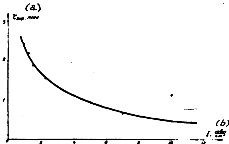
Fig. 2. Recording time as a function of intensity of the exciting radiation. KEY: (a) ms (b) \frac{mW}{cm^2}
